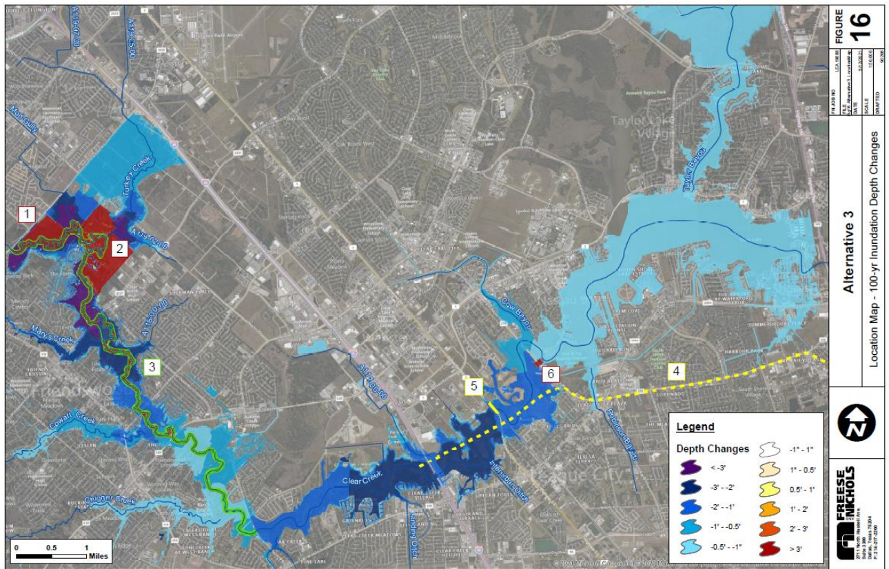
FIGURE 5-2: ALTERNATIVE 3 LOCATION AND INUNDATION DEPTH CHANGE MAP
