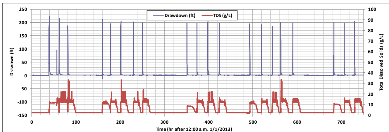
Figure 1. Depth to water and total dissolved solids variations during January, 2013
