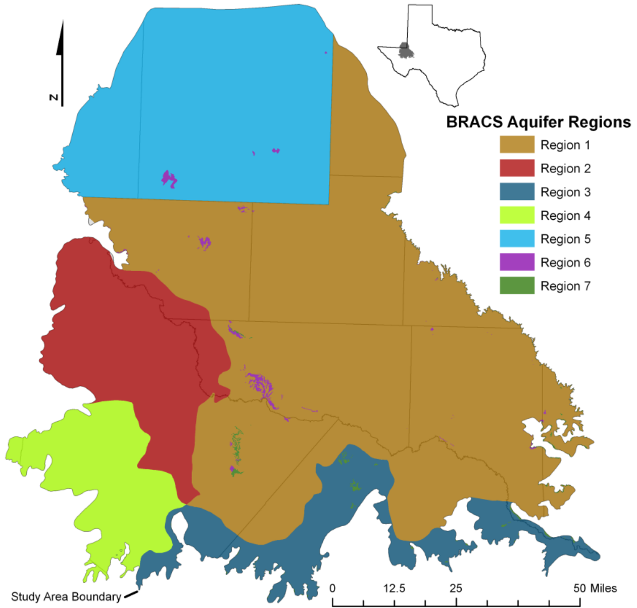
Figure 16.1-1. Regions within the Pecos Valley Alluvium study area. Refer to Table 16.1-2 for the stratigraphic sequence within each region.
