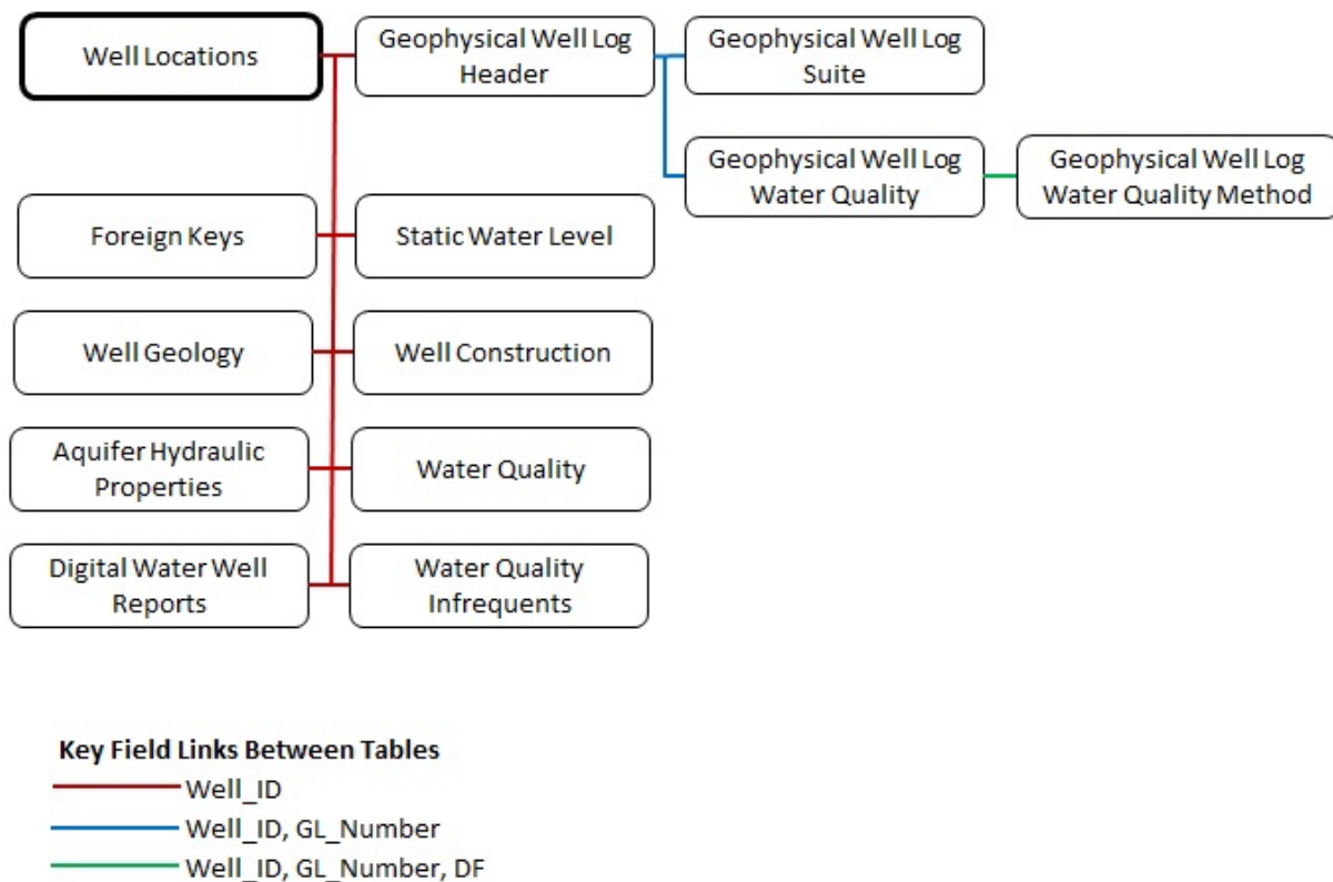
Figure 1-1. BRACS Database table relationships. Each rectangle represents the type of information in a primary table and the link(s) to the other tables based on key fields, represented by colored lines. The Well Location table, in bold outline, is the primary table where the well record identification number, Well_ID, is assigned.
