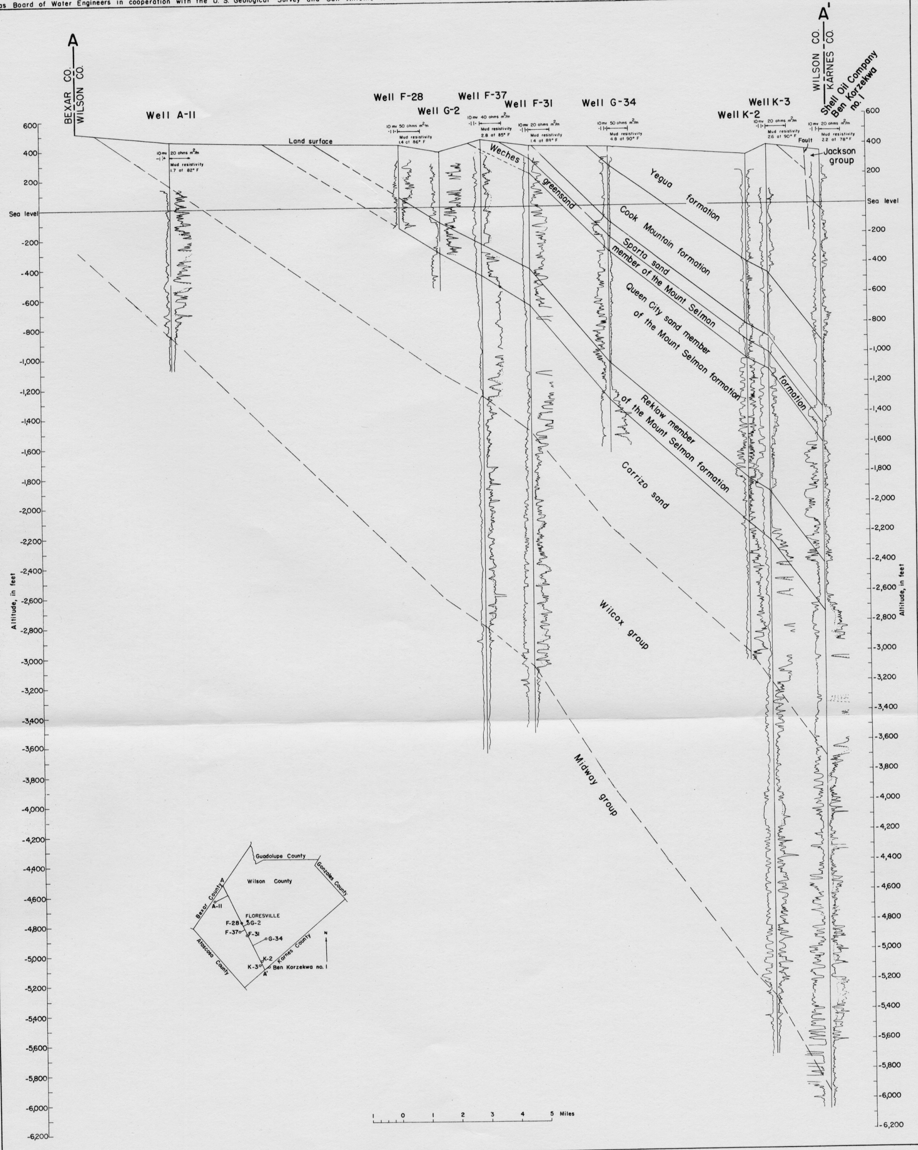
GEOLOGIC CROSS SECTION A-A', WILSON COUNTY, TEXAS
