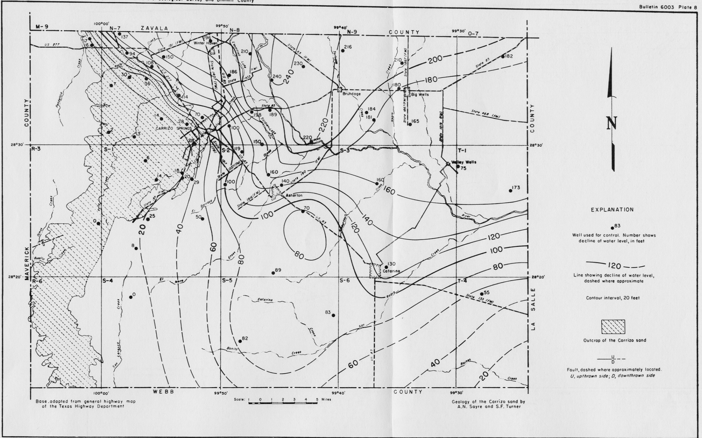
DECLINE OF WATER LEVELS IN WELLS IN THE CARRIZO SAND, DIMMIT COUNTY, TEXAS, 1929-57.
