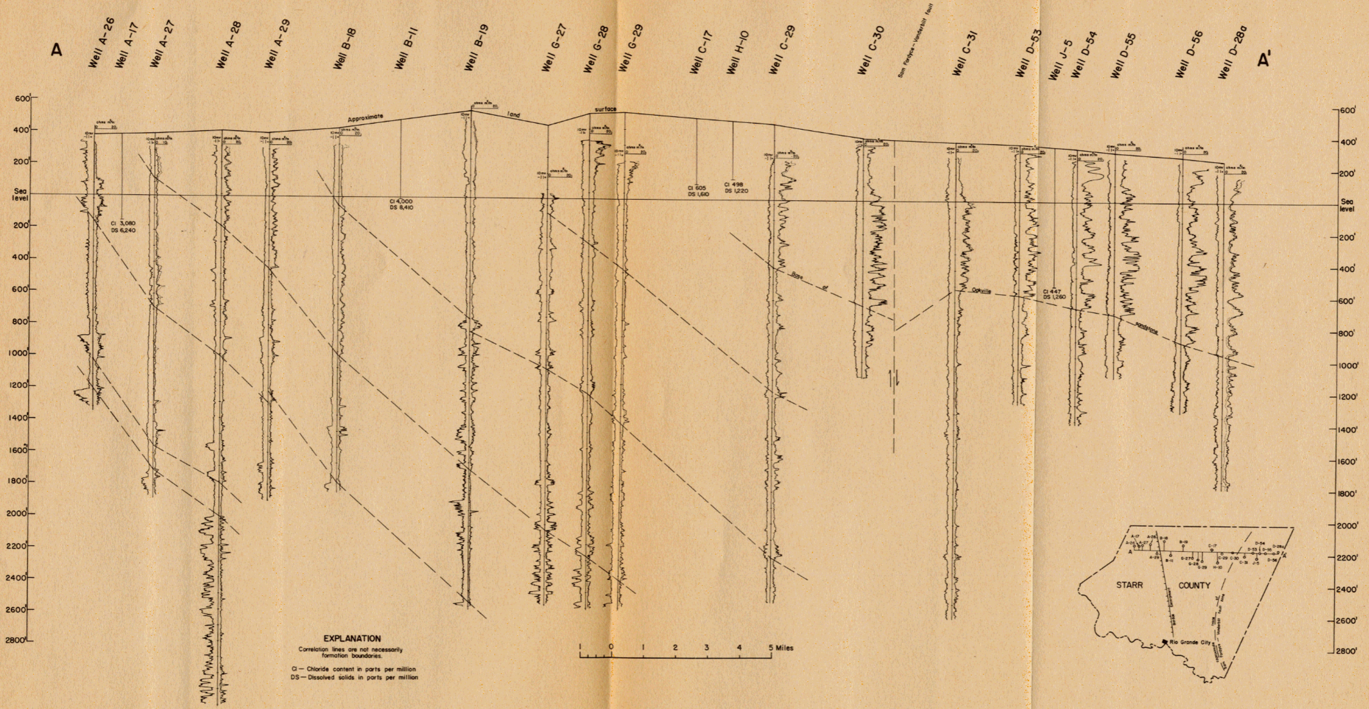
GEOLOGIC SECTION A-A', STARR COUNTY, TEXAS
