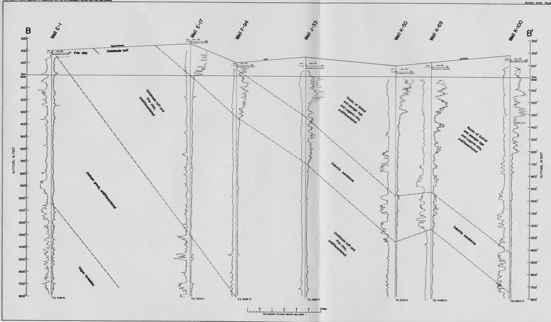
GEOLOGIC SECTION B-B', LIVE OAK COUNTY
