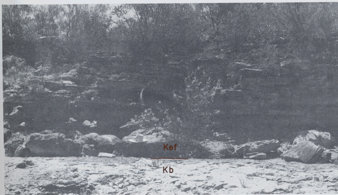
B. CONTACT OF THE EAGLE FORD SHALE (Kef) AND BUDA LIMESTONE (Kb) IN SOUTH BANK OF PINTO CREEK, 6-1/2 MILES NORTHWEST OF BRACKETTVILLE
