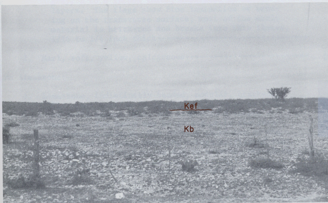
A. VEGETATIONAL CHANGE BETWEEN EAGLE FORD SHALE (Kef) AND BUDA LIMESTONE (Kb), ABOUT 5 MILES NORTH OF BRACKETTVILLE AT WEST SIDE OF SILVER LAKE ROAD
