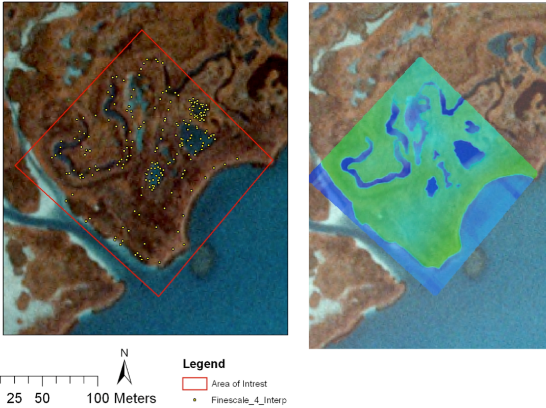
Figure A4: GIS maps showing the location of survey points at Sundown Bay creek and marsh (left) and interpolated elevation, which can then be used to simulate water level rise and connectivity at a small scale (right).
