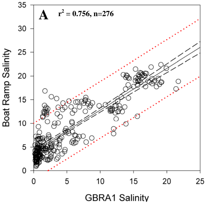
Figure 3.5. Relationship between salinities (ppt) of the tidal creeks sampled in each whooping crane territory ((A) Boat Ramp, (B) Pump Canal and (C) Sundown Bay) and salinities recorded at the GBRA1 gauge in San Antonio Bay. Black lines represent trend lines from linear regression (with associated r^2 and sample sizes (n)). Black dashed and red dotted lines represent 95% confidence and prediction intervals, respectively. Data were collected from 24 February 2004 to 25 February 2005.
