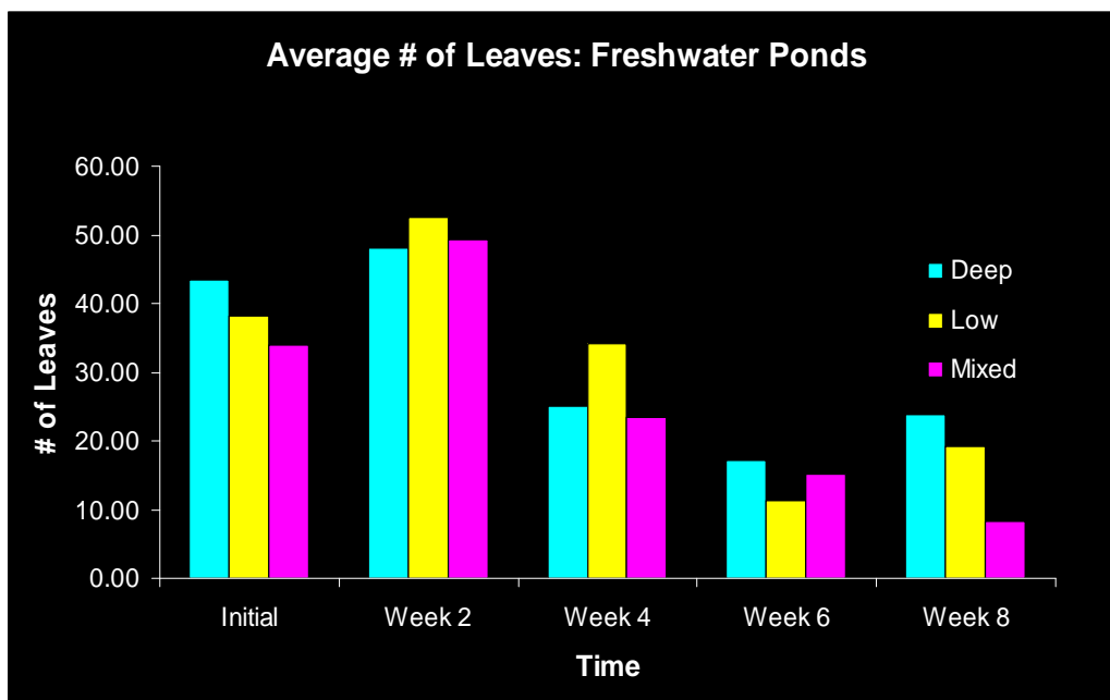
Figure A5: Graphs depicting the change in the total number of leaves over the course of the 8-week experiment in both the saltwater (top) and freshwater (bottom) ponds. Inundation treatments of deep, low, and mixed are shown as different colors.
