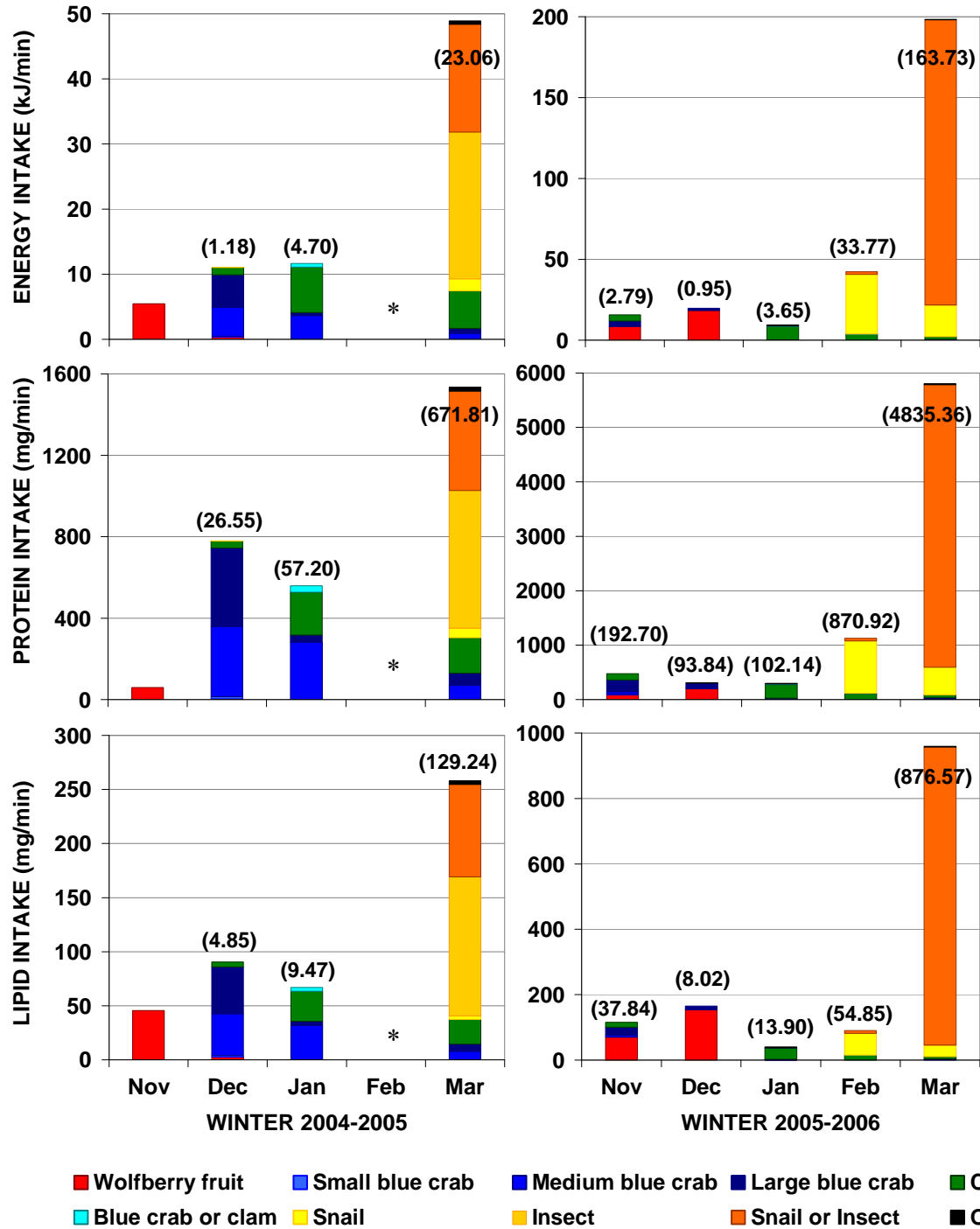
Figure A21. Contribution of foods to mean energy, protein, and lipid intake rates for whooping cranes during each month of winters 2004-2005 and 2005-2006. Standard errors (in parentheses) represent variability among territories ( n = 3 territories for all months, except n = 1 territory in Nov 2004). No data were collected in February 2005 (*). Note large differences in scales of y-axis between winters.
