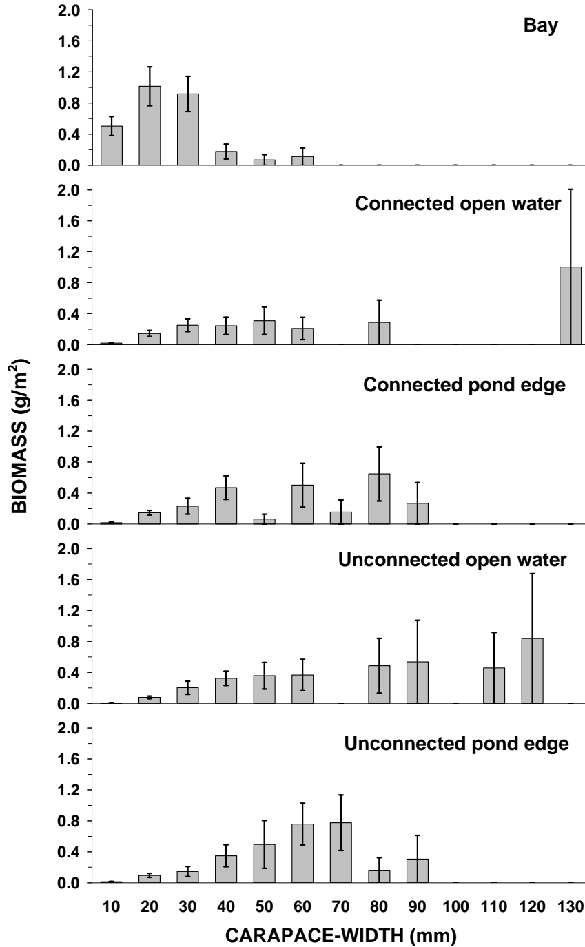
Figure A9. Mean biomass (g/m 2 ) of crabs by carapace-width for each habitat, averaged over all months sampled between October 2004-March 2006. Crabs are grouped by increments of 10 mm, the upper bounds of which are noted along the x-axis. Error bars represent variability in densities among months ( \pm 1 SE).
