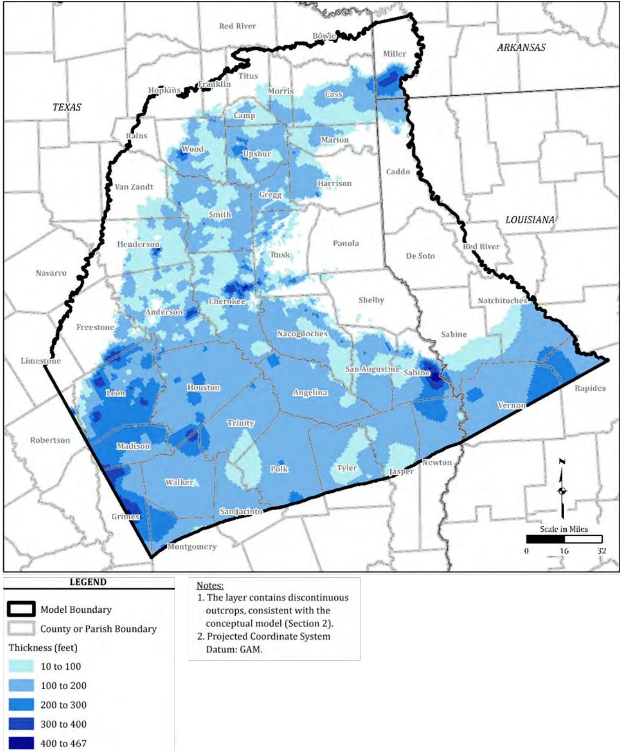
Figure 2.4-15. Modeled Thickness for Carrizo Aquifer (Model Layer 6)
