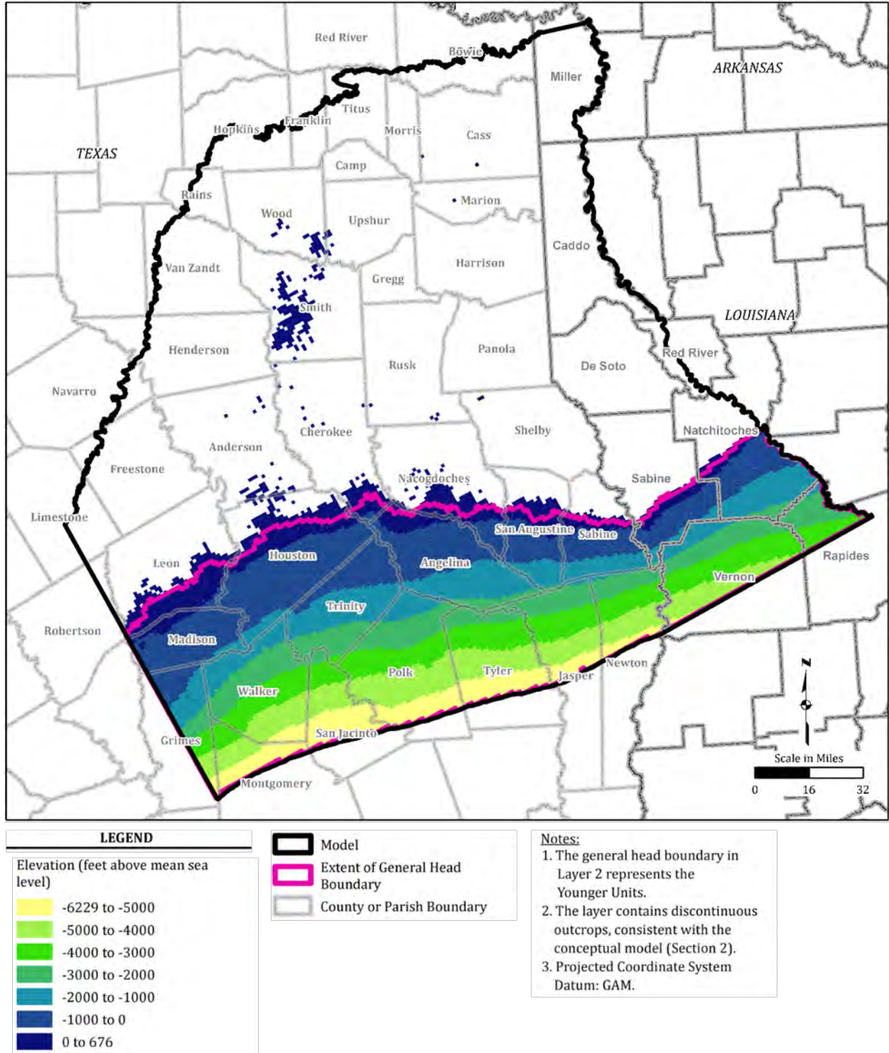
Figure 2.4-5. Modeled Top Elevation for Sparta Aquifer (Model Layer 2)
