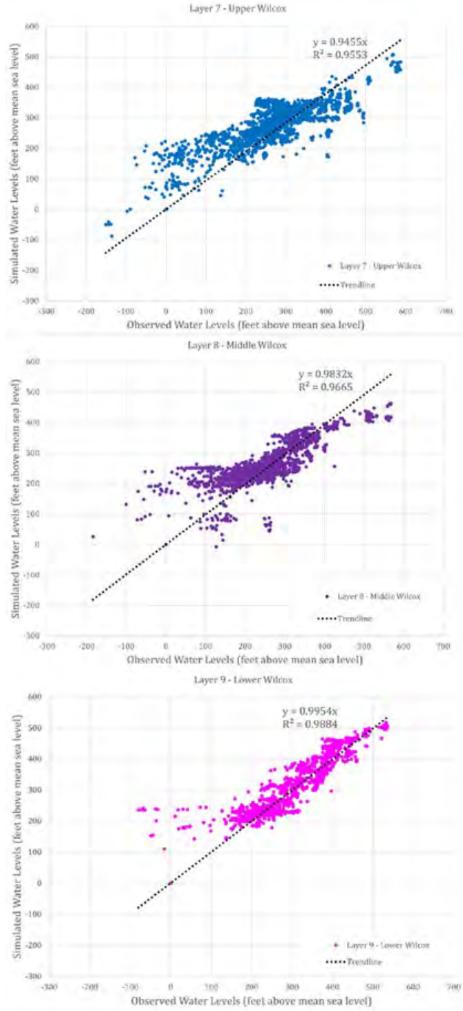
Figure 3.2-15c. Observed vs. Simulated Water Level Elevations for Calibrated 1980 to 2013 Simulation by Layer
