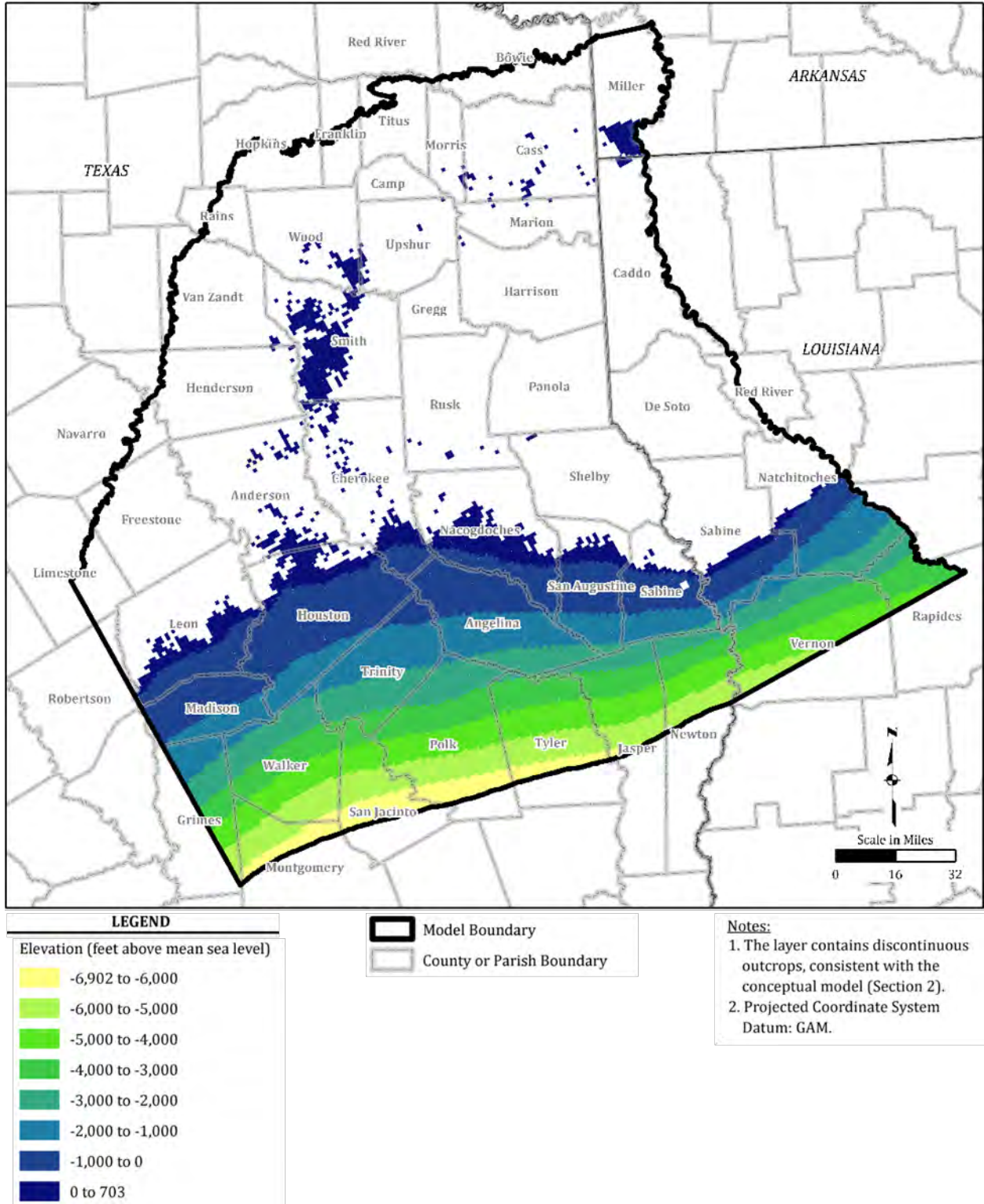
Figure 2.4-8. Modeled Bottom Elevation for Weches Formation (Model Layer 3)
