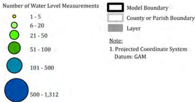
Figure 3.2-7. Location of Groundwater Observation Wells and Available Water Level Elevation Data - Lower Wilcox (Layer 9)
