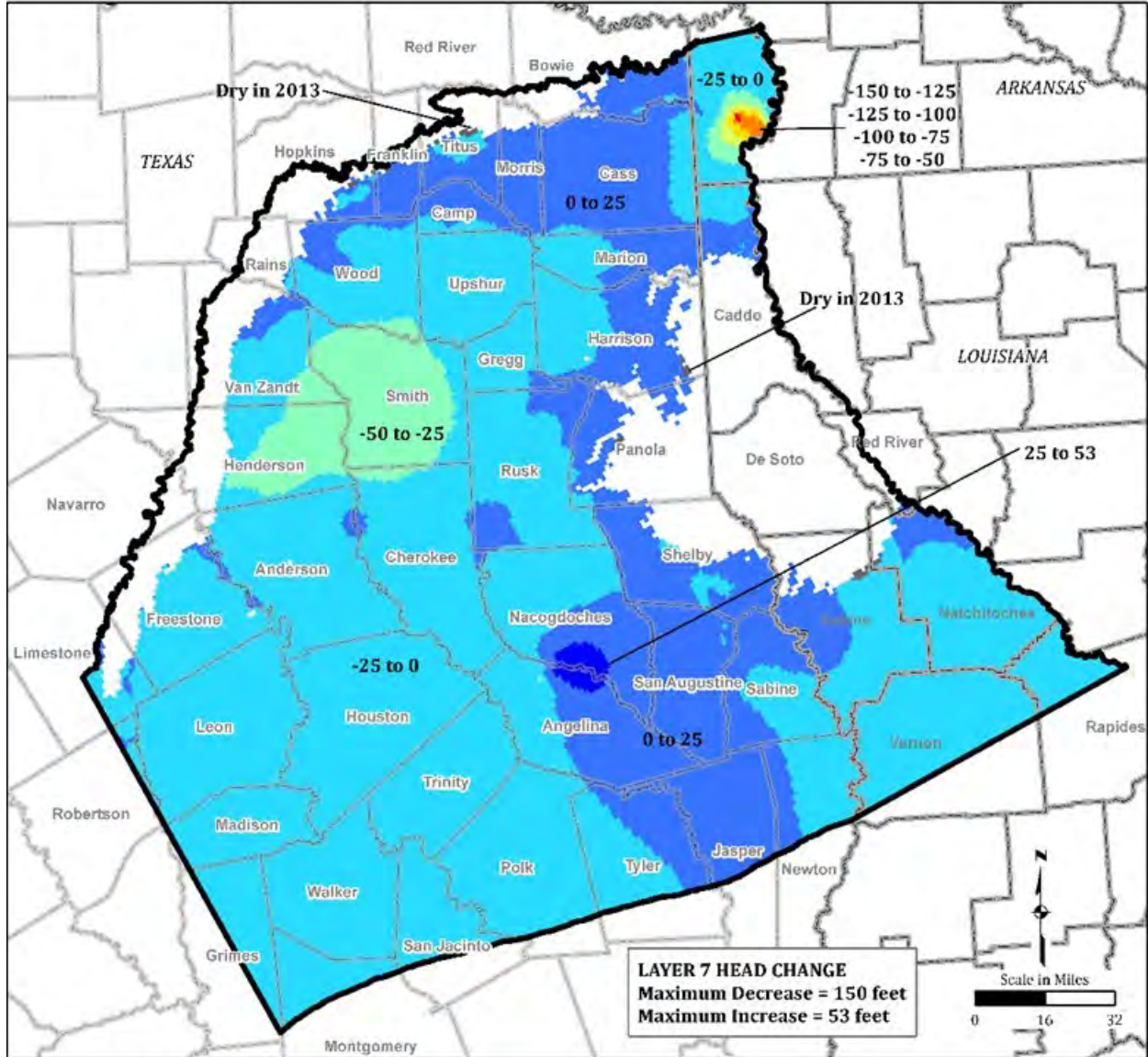
LEGEND Head Change from 1980 to 2013 (feet) Model Boundary County or Parish Boundary Cell is dry in 2013 Notes: The layer contains discontinuous outcrops, consistent with the conceptual model (Section 2). Projected Coordinate System Datum: GAM. Figure 3.2-40. Change in Water Level Elevations Between 1980 and 2013 in Upper Wilcox (Layer 7)
