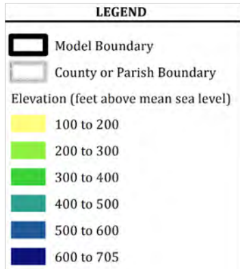
Figure 2.4-2. Modeled Top Elevation for Quaternary Alluvium (Model Layer 1)
