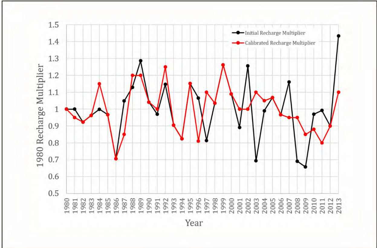
Figure 2.10-2. Model Precipitation Multipliers 1980 to 2013
