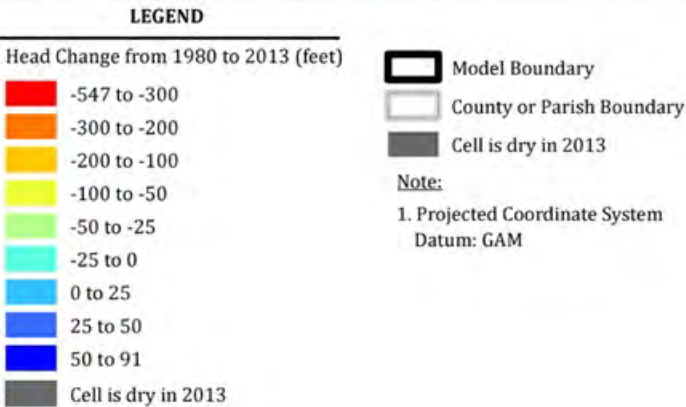
Figure 3.2-41. Change in Water Level Elevations Between 1980 and 2013 in Middle Wilcox (Layer 8)
