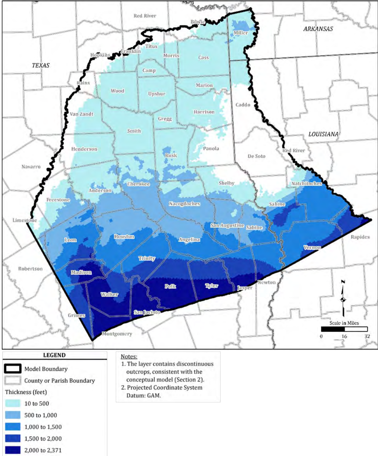
Figure 2.4-17. Modeled Thickness for Upper Wilcox (Model Layer 7)
