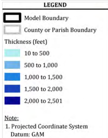
Figure 2.4-21. Modeled Thickness for Lower Wilcox (Model Layer 9)
