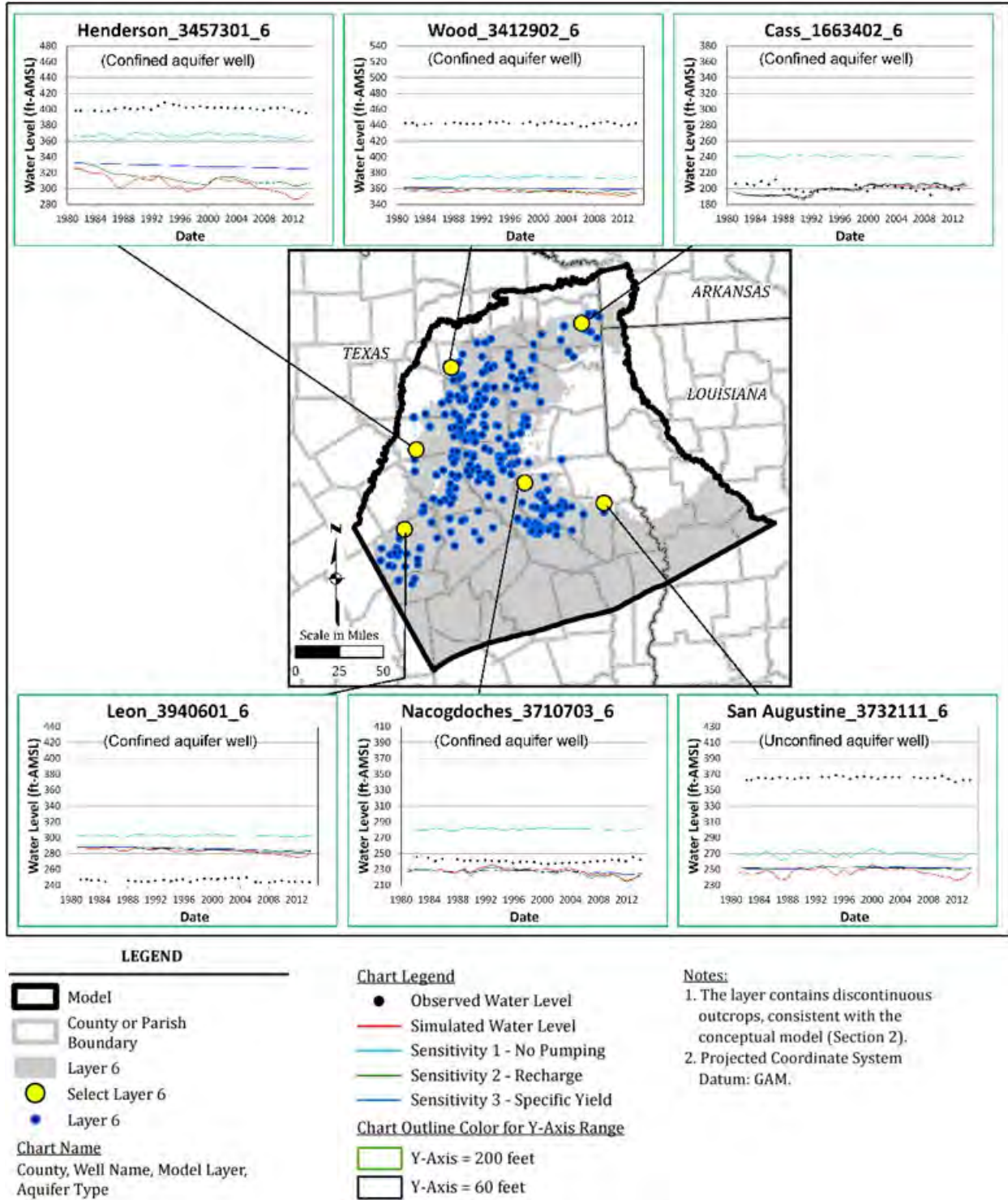
Figure 4.2-10. Measured and Simulated Hydrographs at Select Wells Showing Model Sensitivity - Carrizo Aquifer (Layer 6)
