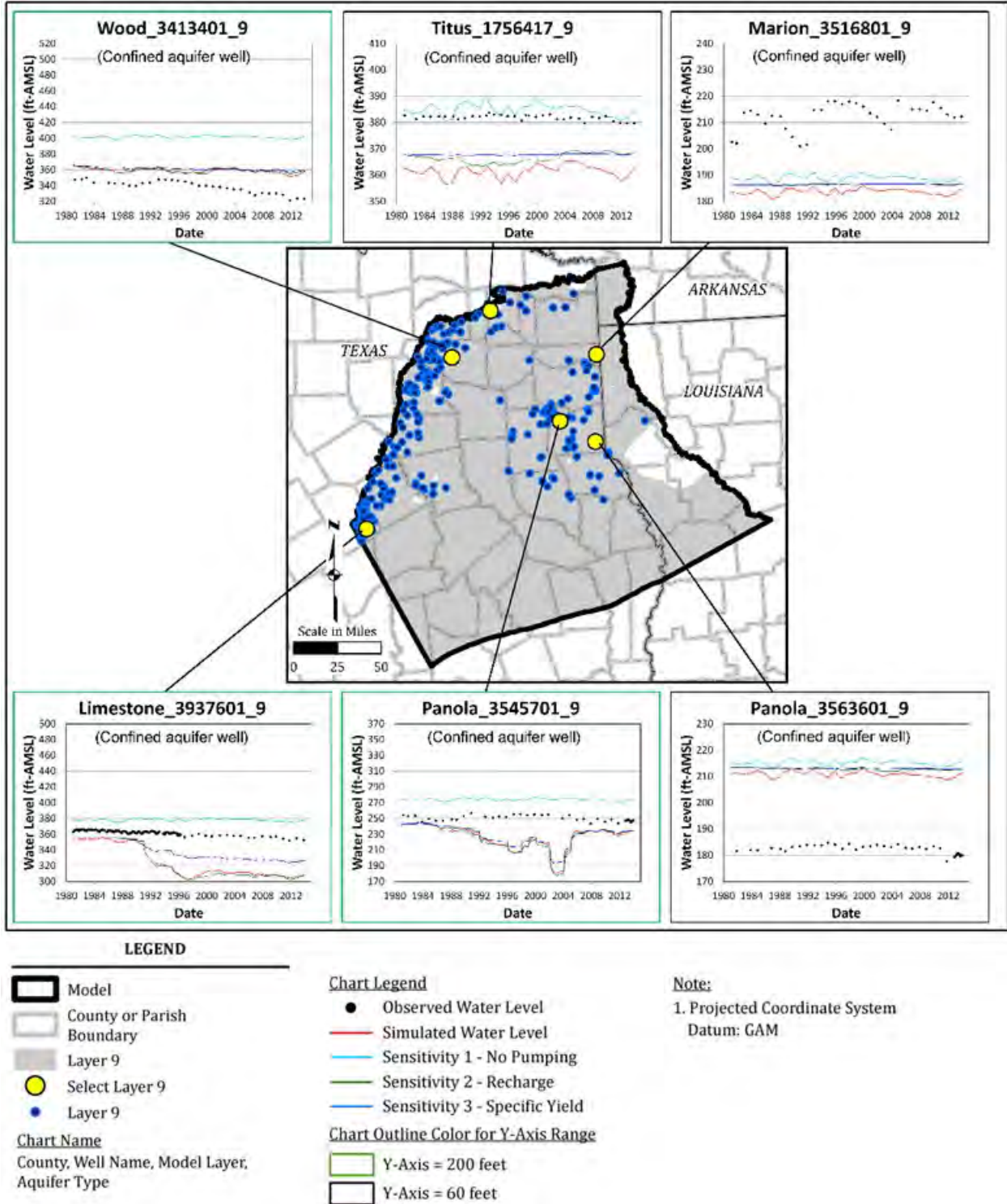
Figure 4.2-13. Measured and Simulated Hydrographs at Select Wells Showing Model Sensitivity - Lower Wilcox (Layer 9)
