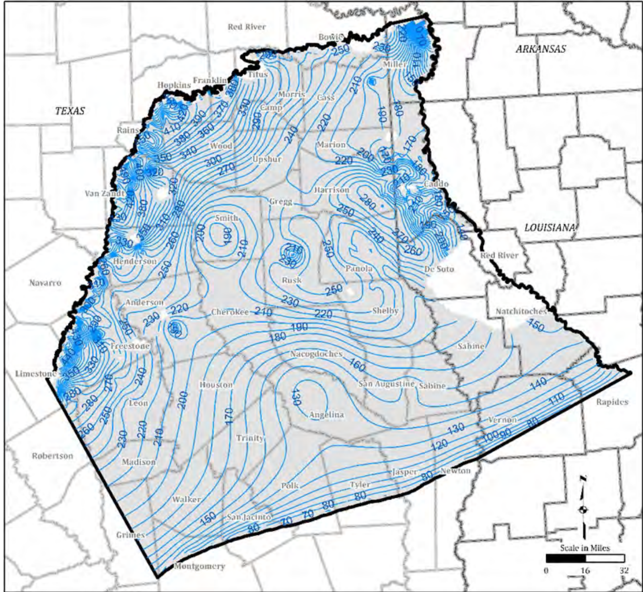
LEGEND — Simulated Water Level — Elevations Contours (feet above mean sea level) ▭ Model ▭ County or Parish ▭ Layer Note: 1. Projected Coordinate System Datum: GAM Figure 3.2-33. Simulated Water Level Elevation Contours in Lower Wilcox (Layer 9) for 2013
