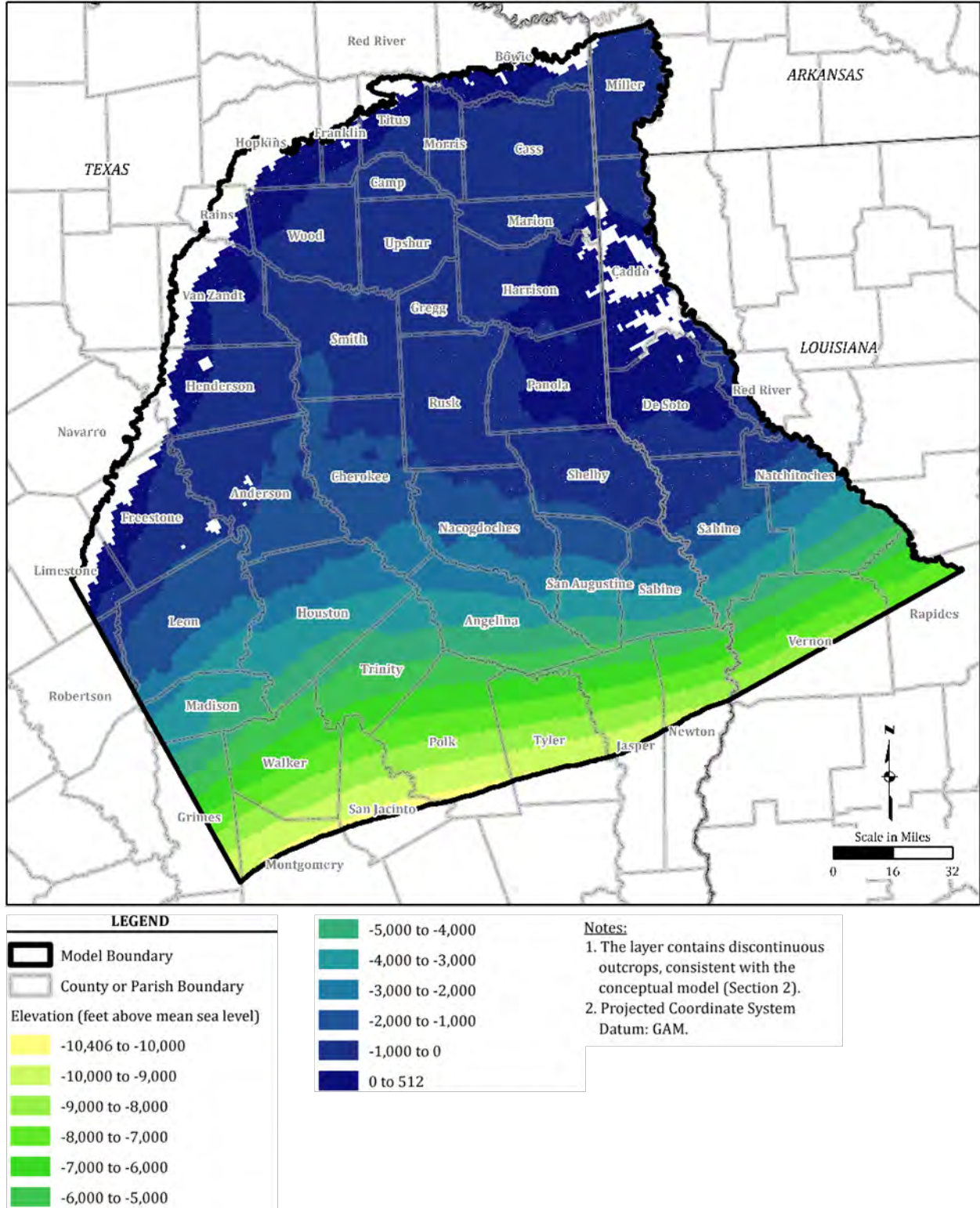
Figure 2.4-18. Modeled Bottom Elevation for Middle Wilcox (Model Layer 8)
