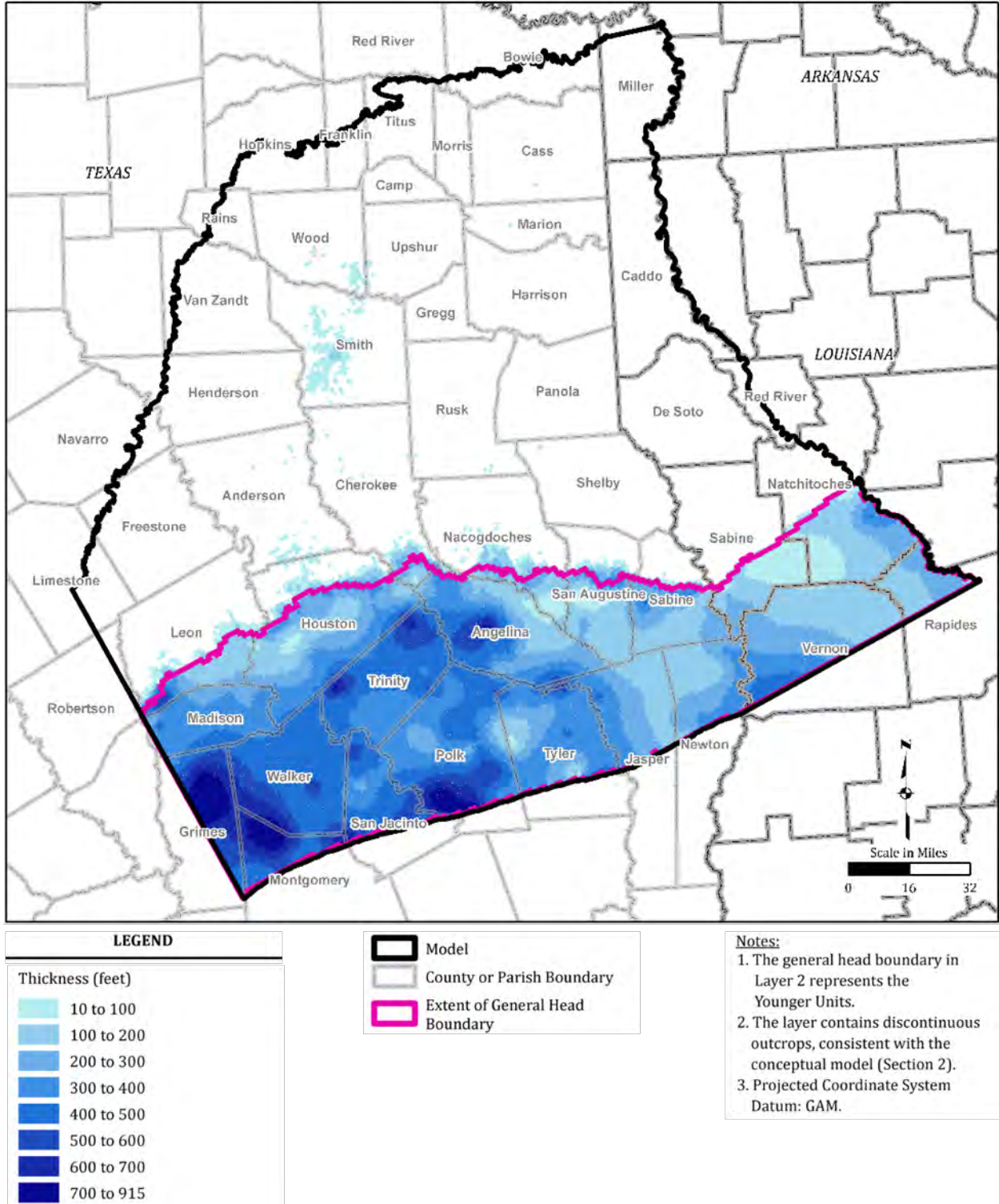
Figure 2.4-7. Modeled Thickness for Sparta Aquifer (Model Layer 2)
