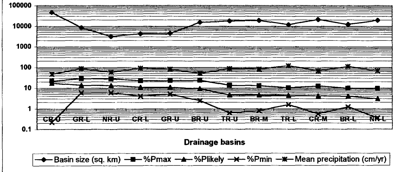
Figure 16: Comparison of the most likely changes in effective precipitation from SIR to basin size and mean precipitation
