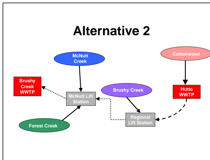
Figure 3-4 Alternative 2 Schematic
