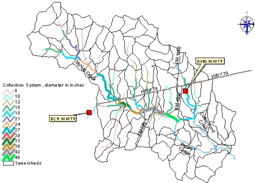
Figure 4-3 Collection System Sizes, Alternative 1, 3
