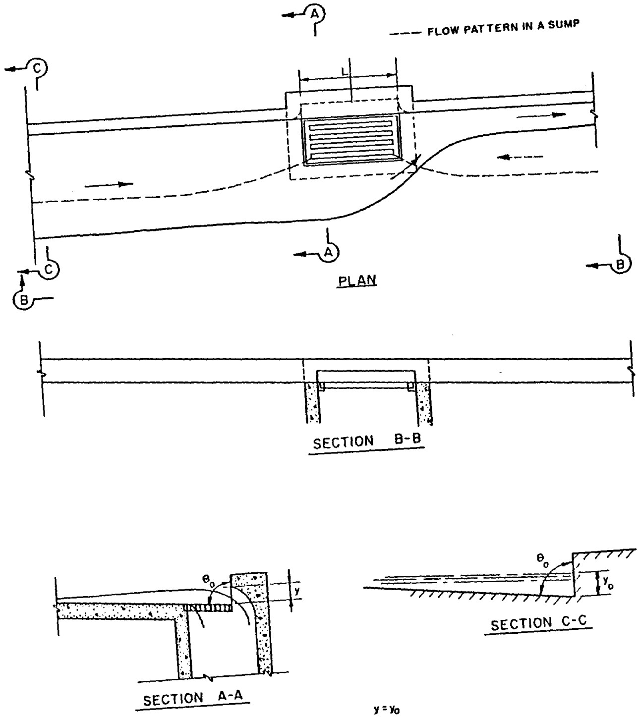
FIGURE 4-8 UNDEPRESSED COMBINATION INLET (RECESSED)
