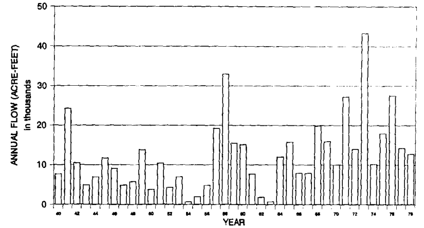
NATURALIZED FLOW IN MIDDLE VERDE CREEK AT PROPOSED DAM SITE
