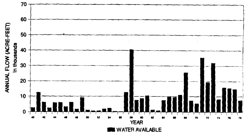
NATURALIZED FLOW IN SECO CREEK AT USGS GAGE 08201500
