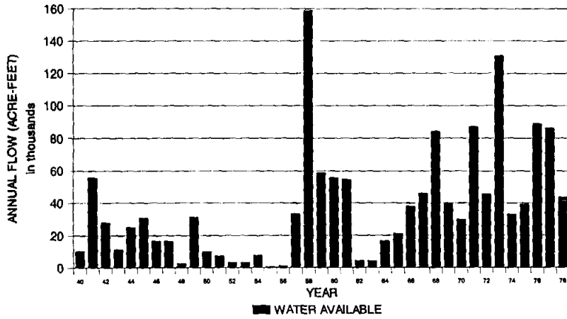
NATURALIZED FLOW IN SABINAL RIVER AT USGS GAGE 08198000
