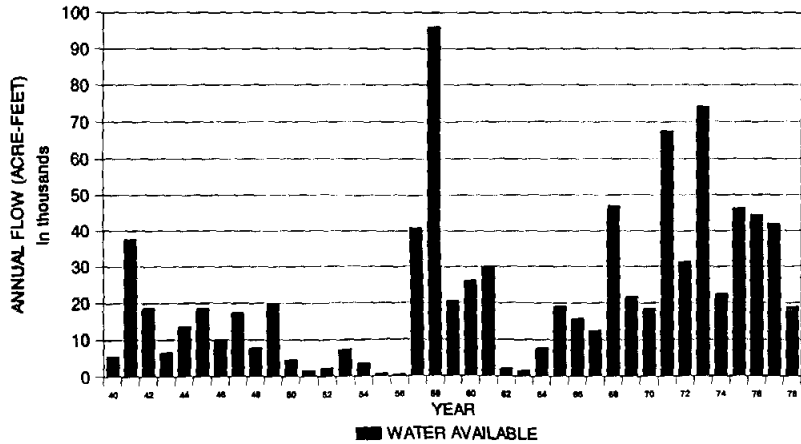
NATURALIZED FLOW IN HONDO CREEK AT USGS GAGE 08200000
