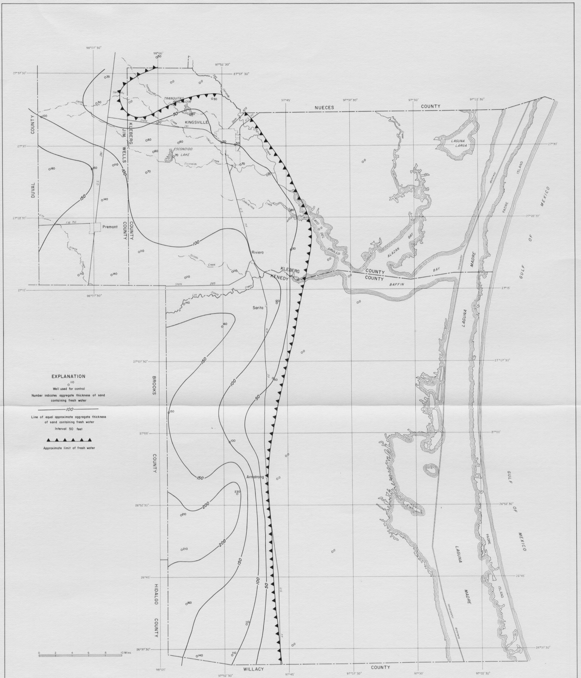
Figure 14 Approximate Thickness of Sand Containing Fresh Water in the Goliad Sand
