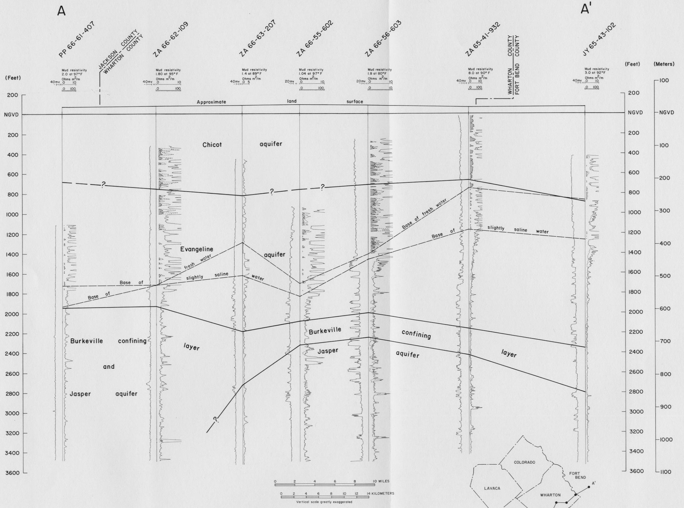
Figure 5 Geohydrologic Section A-A', Jackson, Wharton, and Fort Bend Counties
