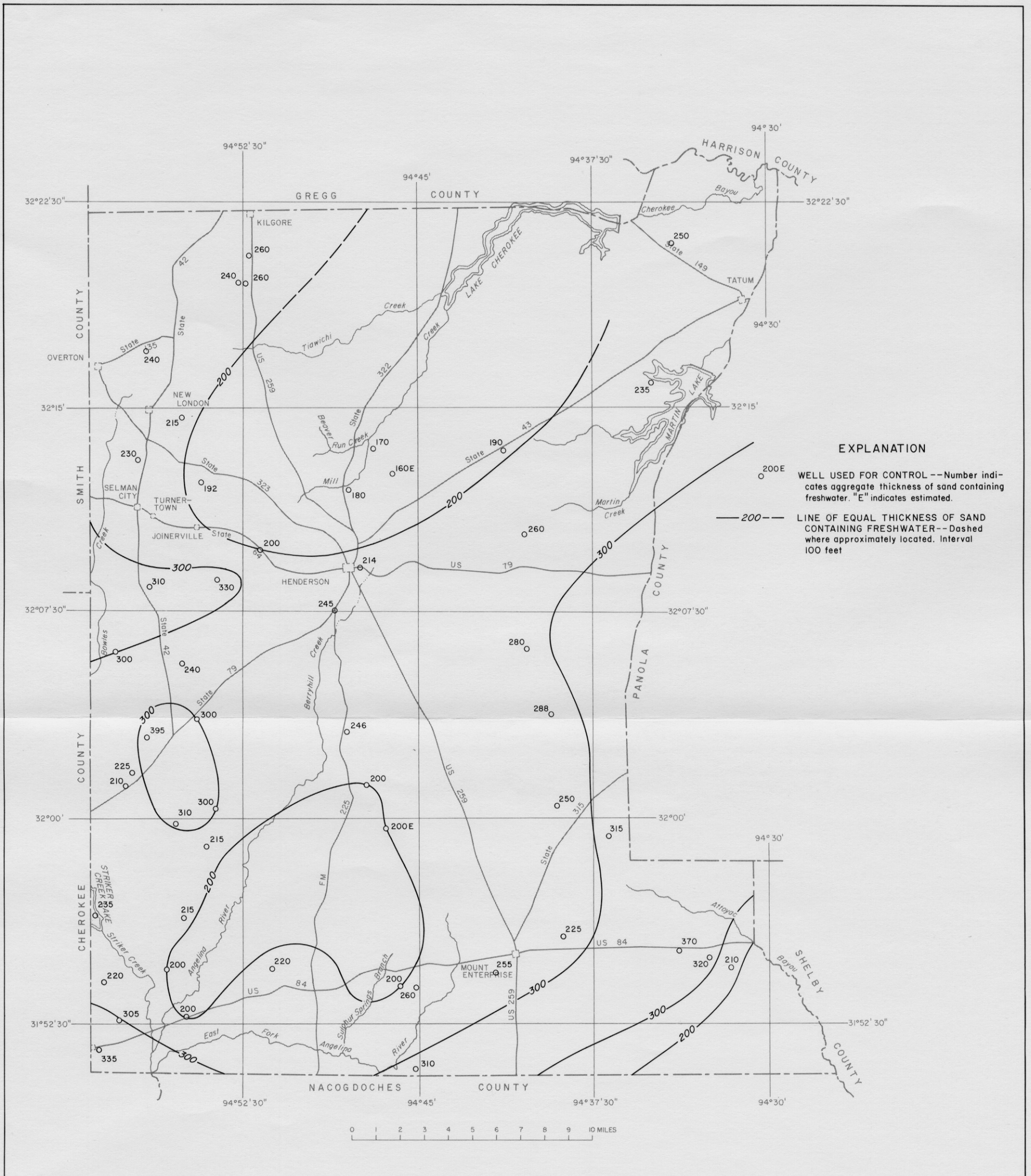
Figure 11 Approximate Thickness of the Freshwater-Bearing Sands in the Wilcox Aquifer, 1981
