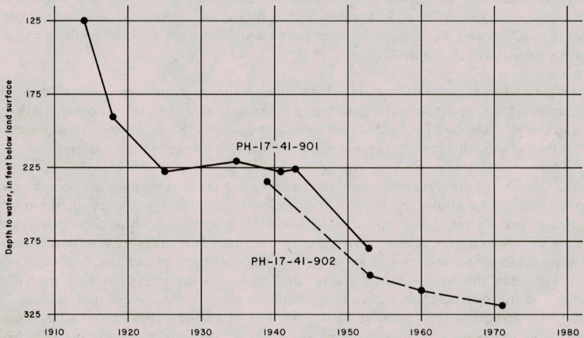
Figure 12.—Hydrographs of Two Public Supply Wells in Commerce, Texas
