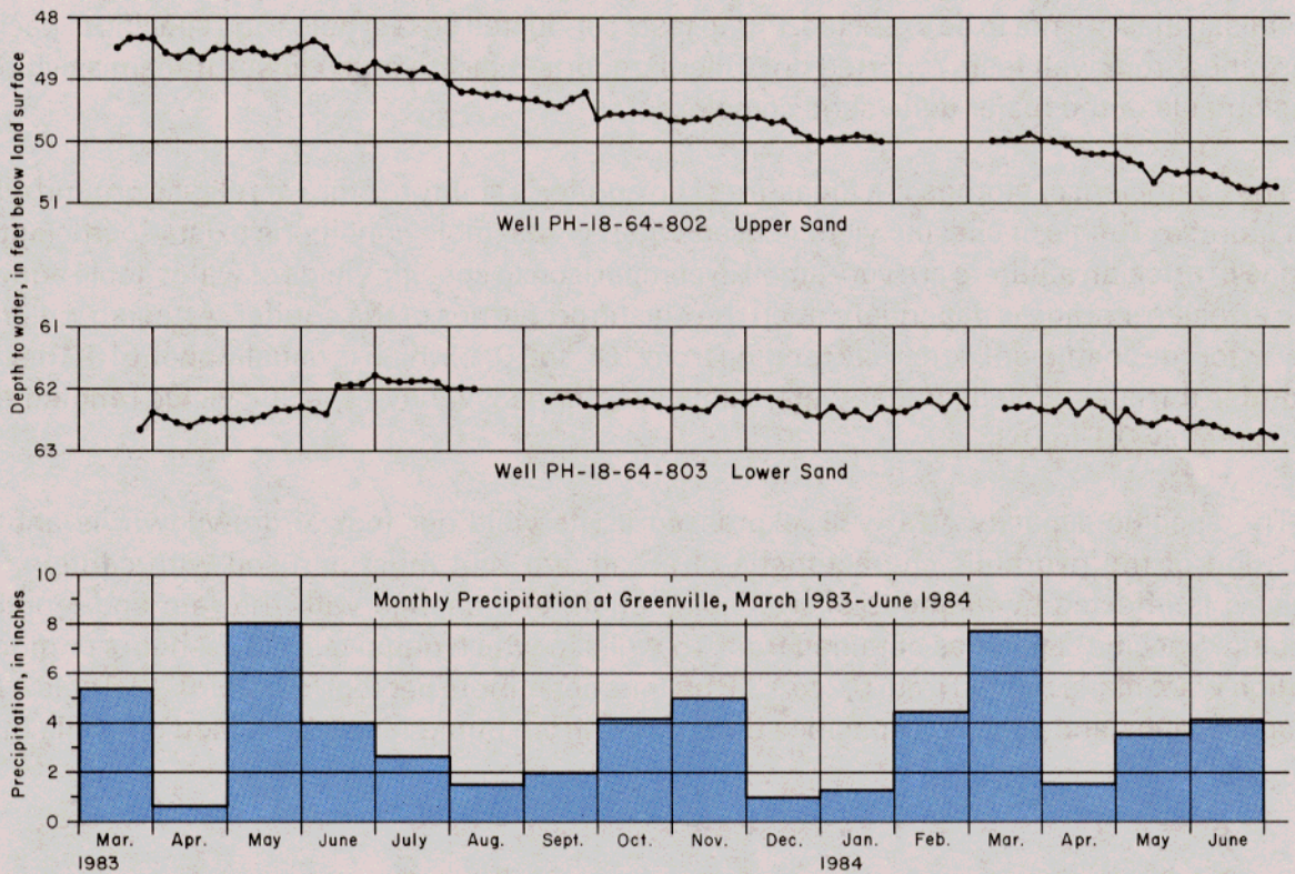
Figure 11.—Hydrographs of Water Levels in Wells Completed in Upper and Lower Nacatoch Sand Units and Monthly Precipitation at Greenville, Texas, March 1983-June 1984
