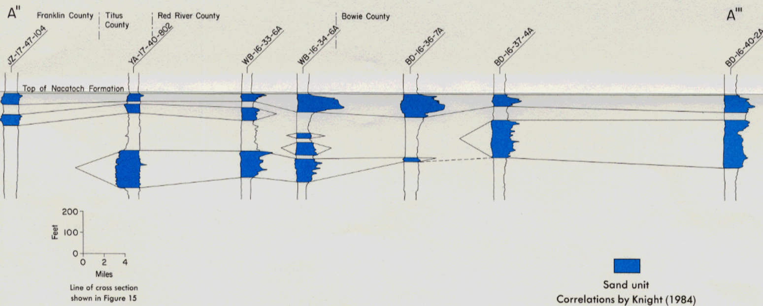
Figure 18 Geologic Section A''-A''' Showing Lateral Correlation of Sand Units
