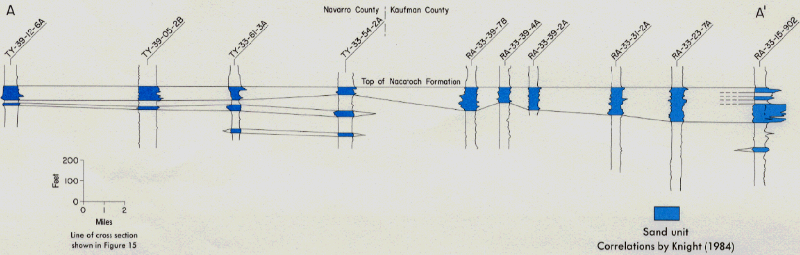
Figure 16 Geologic Section A-A' Showing Lateral Correlation of Sand Units
