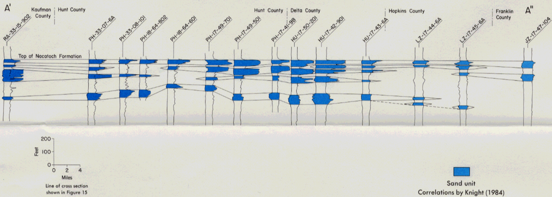
Figure 17 Geologic Section A'-A'' Showing Lateral Correlation of Sand Units
