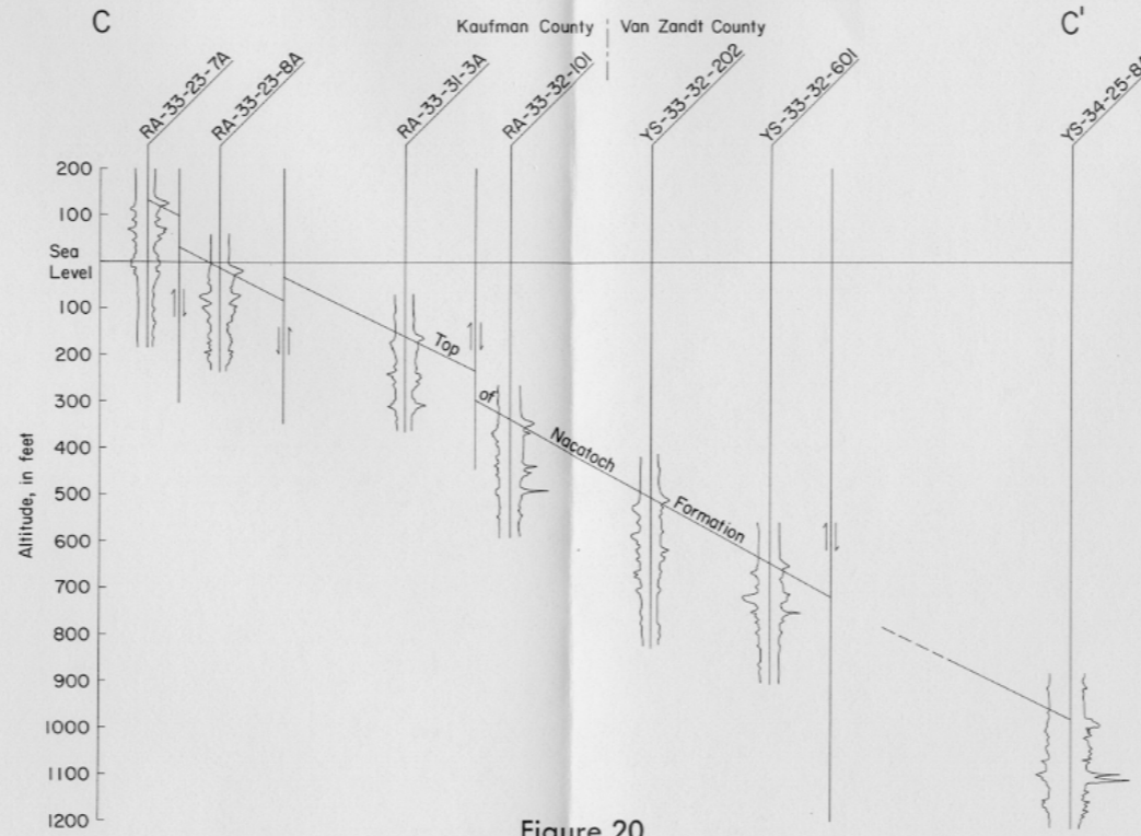
Figure 20 Geologic Section C-C'
