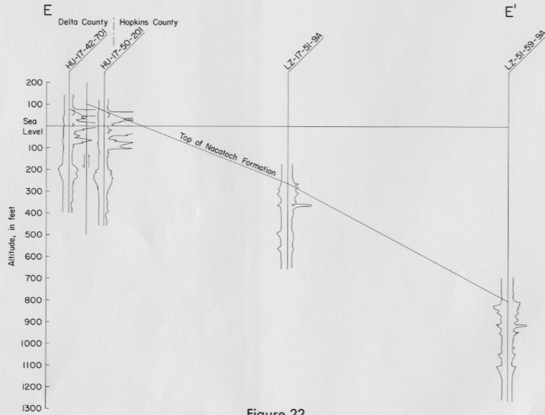
Figure 22 Geologic Section E-E'
