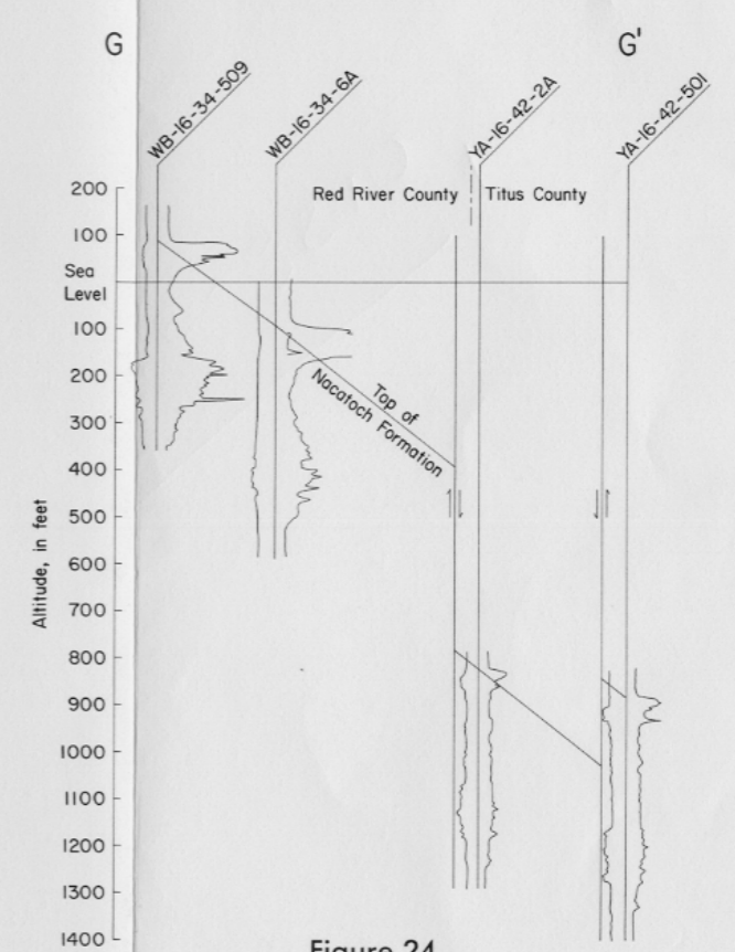
Figure 24 Geologic Section G-G'
