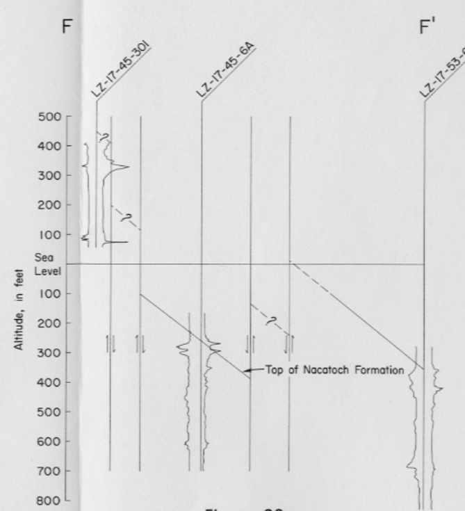
Figure 23 Geologic Section F-F'
