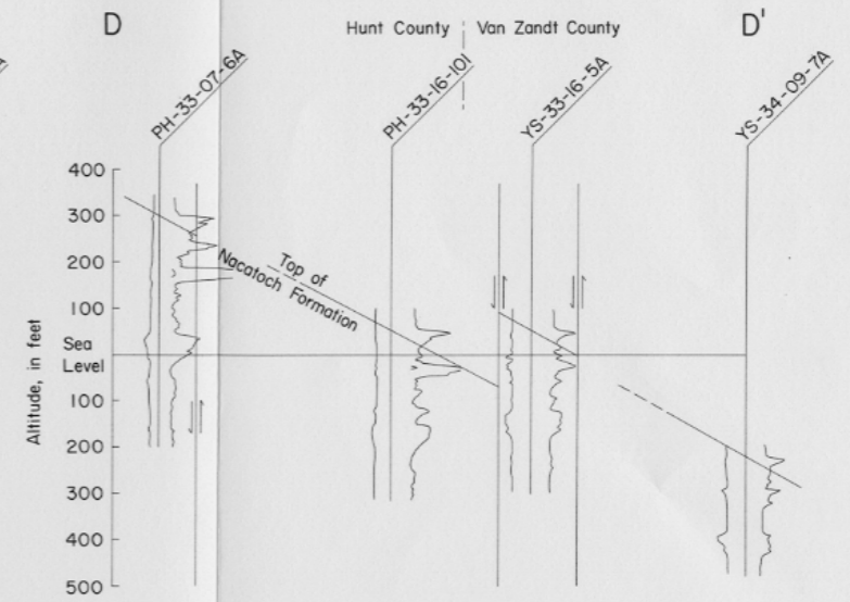
Figure 21 Geologic Section D-D'
