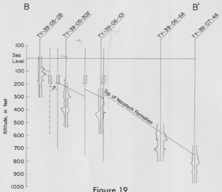
Figure 19 Geologic Section B-B'
