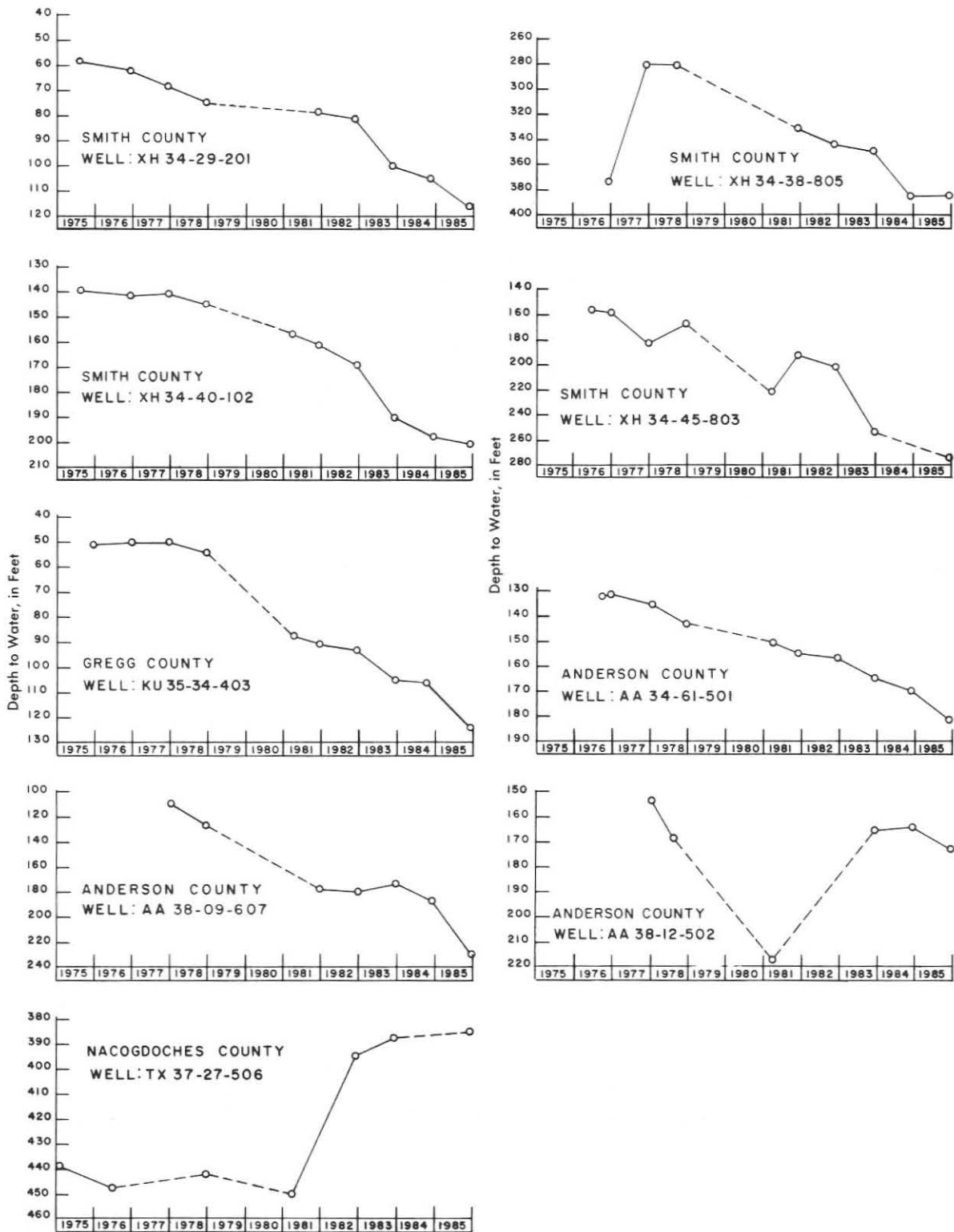
Figure 7 Hydrographs of Selected Wells Completed in the Carrizo-Wilcox Aquifer in Northeast Texas (Well locations shown on Figure 5)
