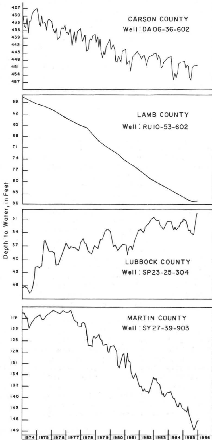
Figure 3 Hydrographs of Selected Wells Completed in the High Plains Aquifer
