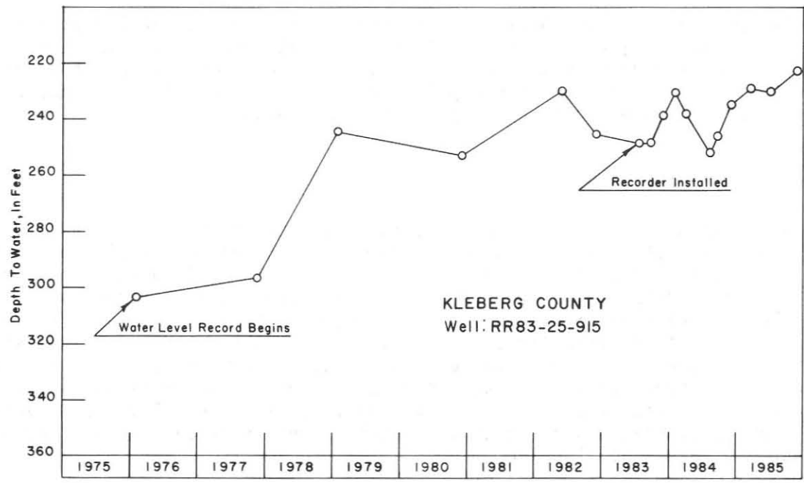
Figure 18 Hydrograph of Well Completed in the Gulf Coast Aquifer in Kingsville in Kleberg County
