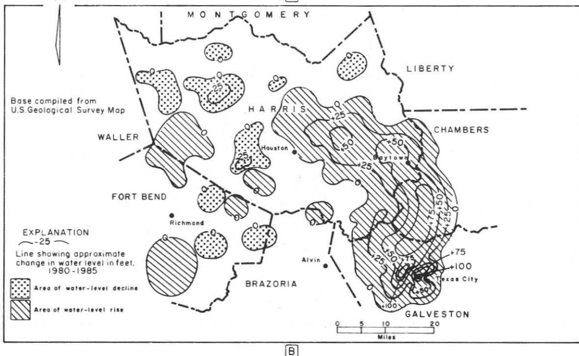
Figure 17 Map Showing Approximate Changes of Water Levels in the Chicot Aquifer for the Periods 1975-85(A) and 1980-85(B)
