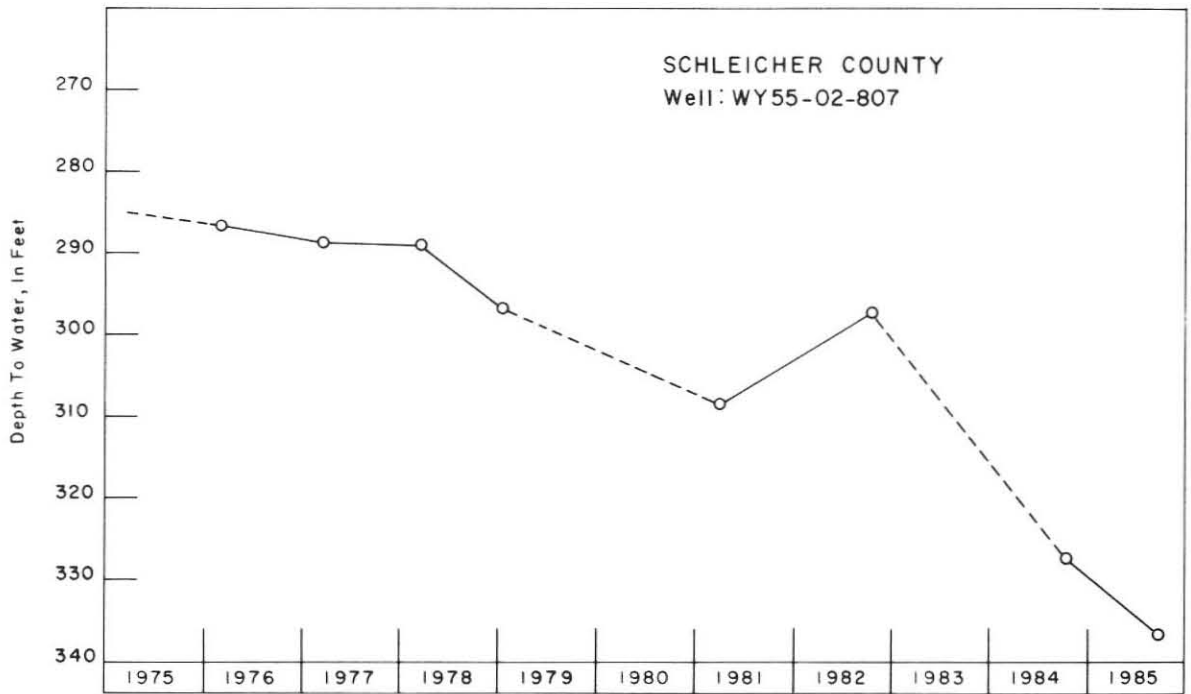
Figure 21 Hydrograph of Well Completed in the Edwards-Trinity Aquifer in Schleicher County
