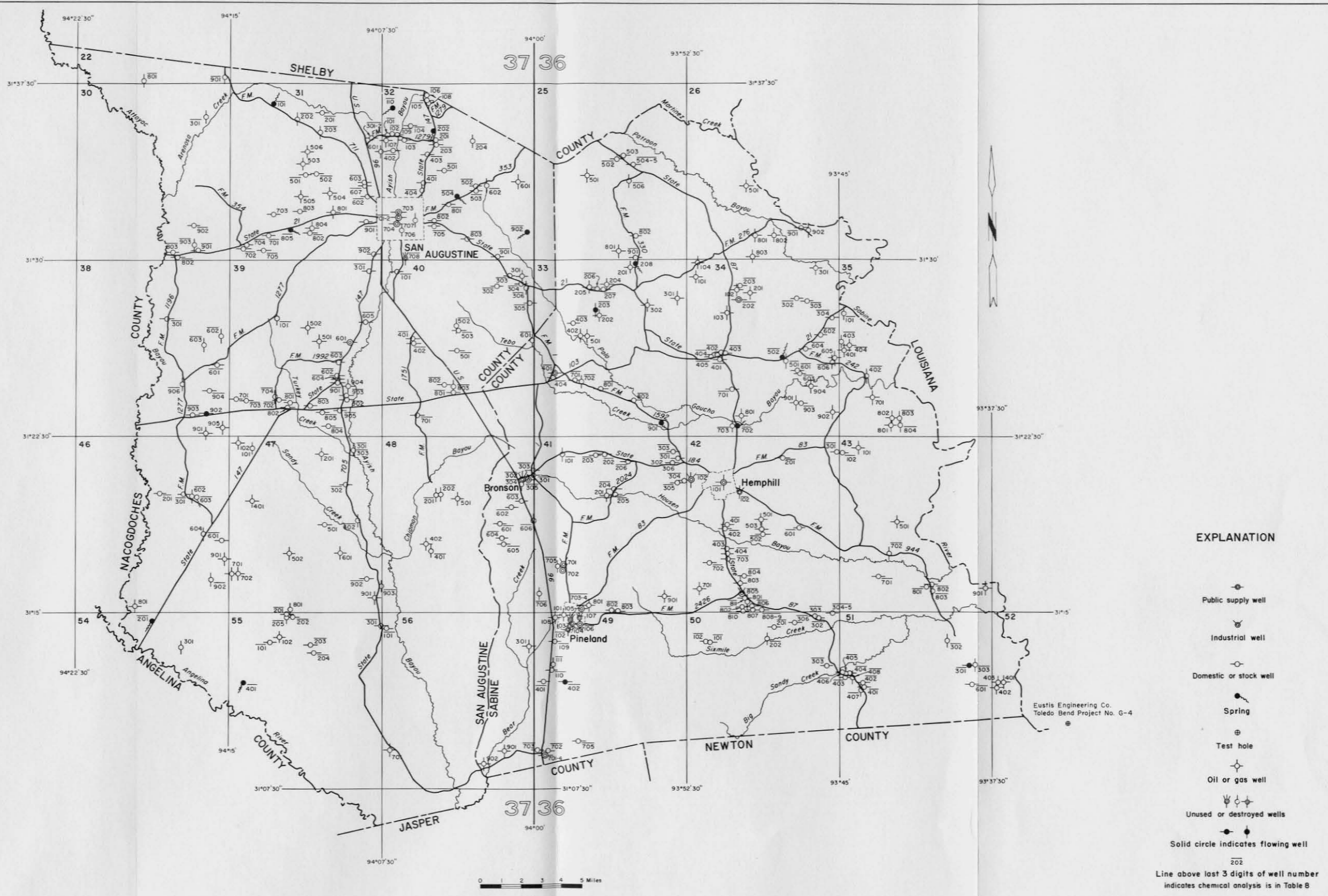
Figure 13 Locations of Wells and Springs
