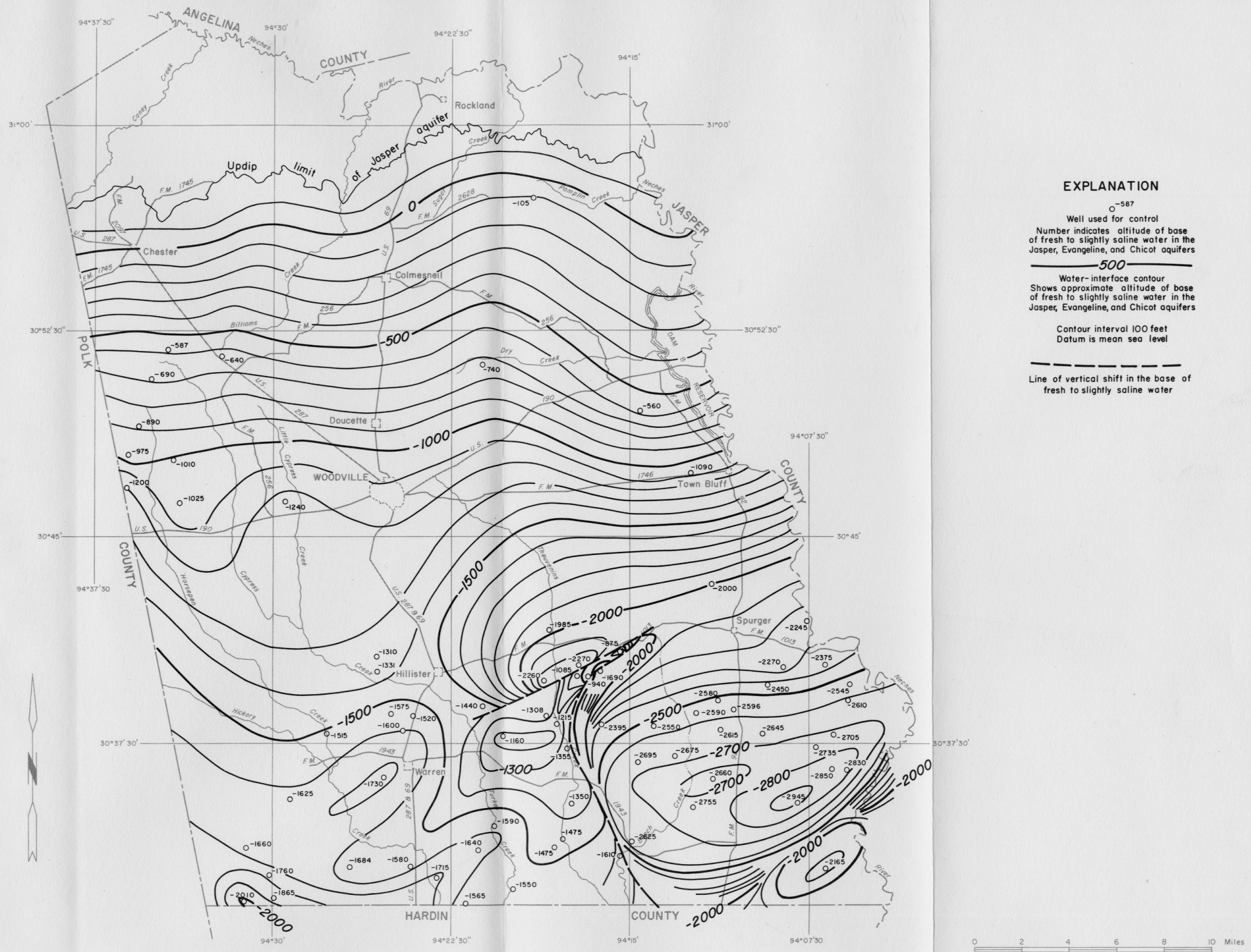
Figure 9 Approximate Altitude of the Base of Fresh to Slightly Saline Water in the Jasper, Evangeline, and Chicot Aquifers
