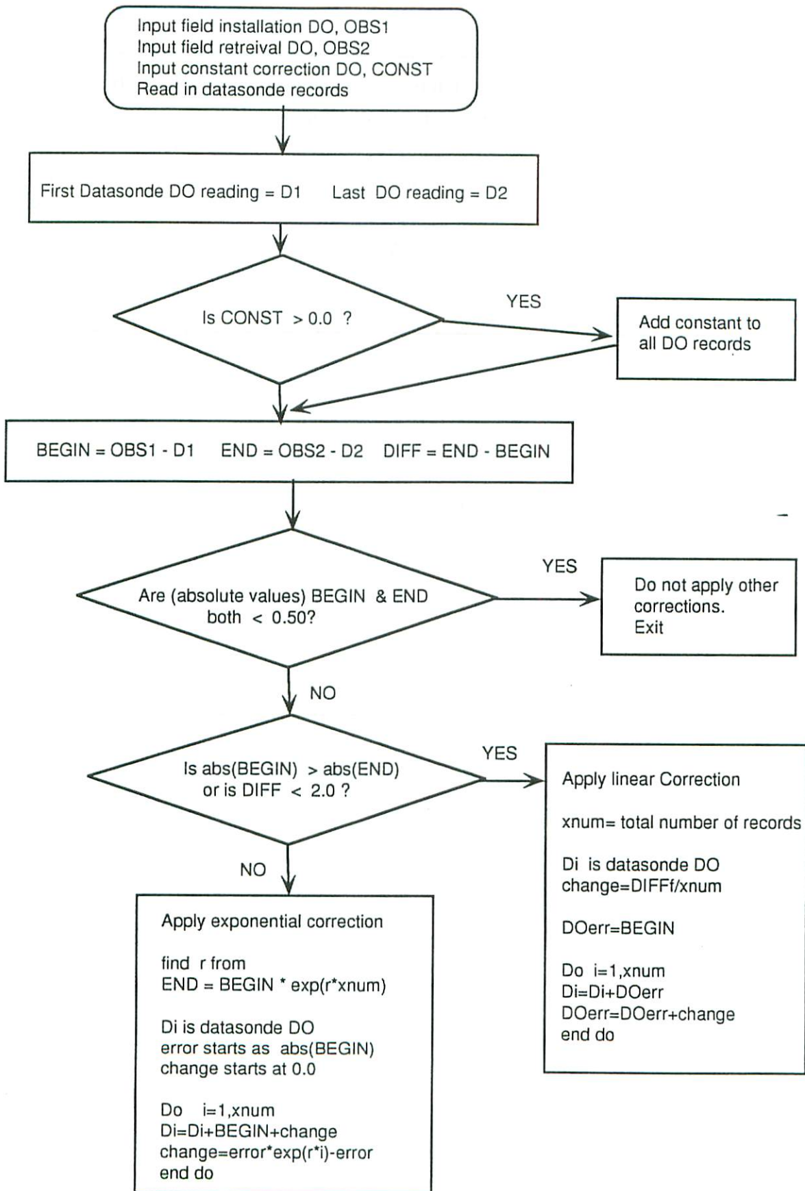
Figure 13. Dissolved oxygen data correction algorithm
