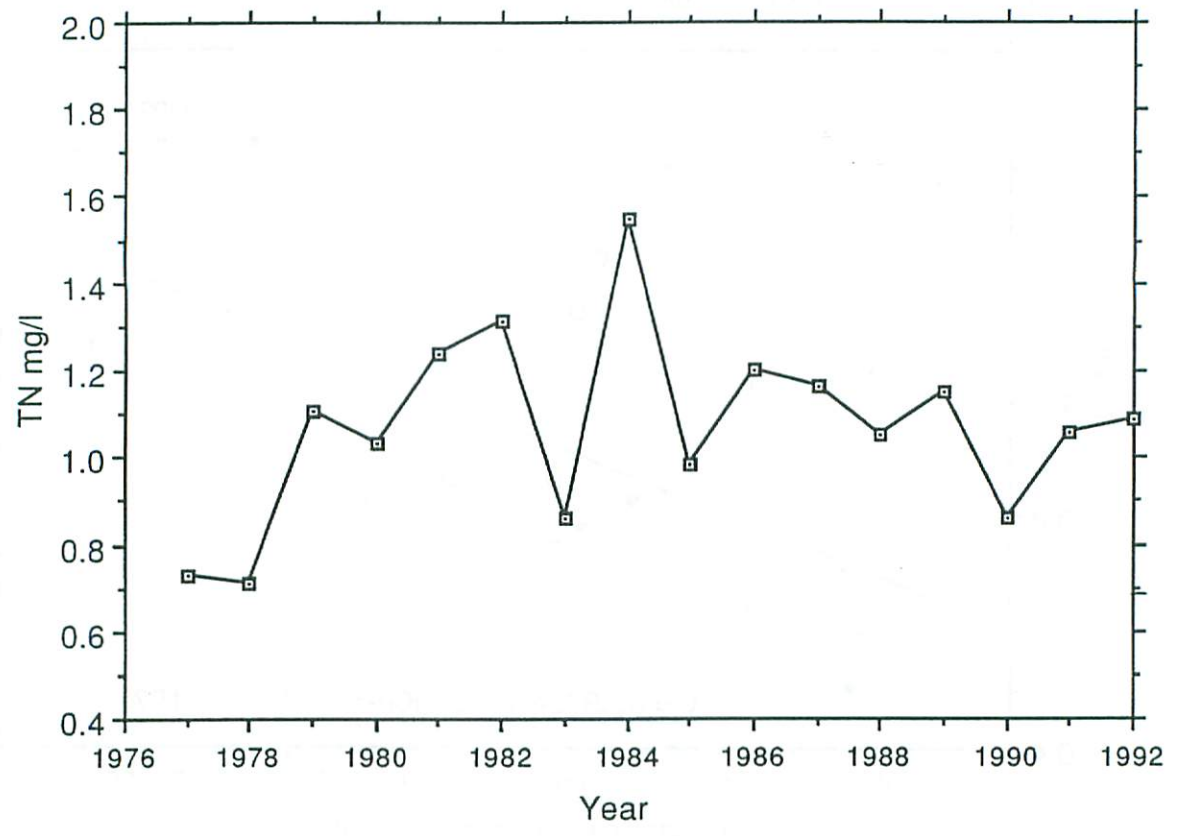
Figure 6. Average TN concentrations in lower Galveston Bay.
