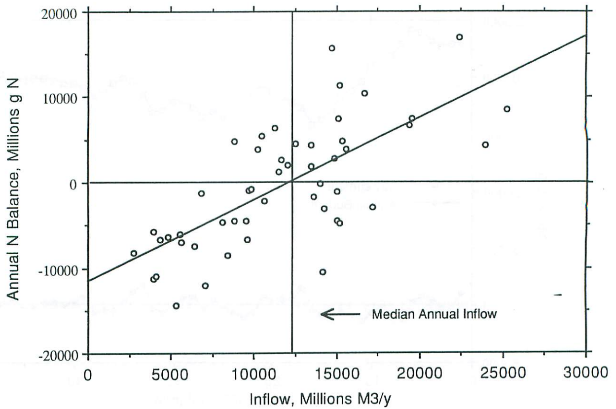
Figure 25. Annual Nitrogen balance from simulations, showing linear fit line and annual inflow at balance = 0.
