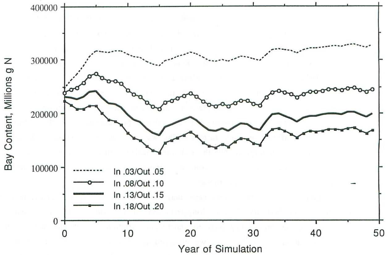
Figure 31. Sensitivity of bay content to tidal mixing rates.
