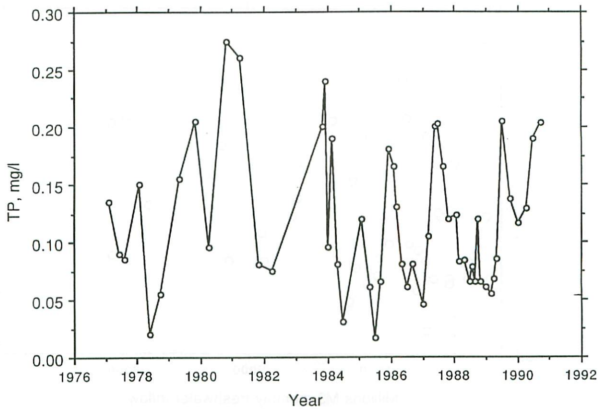
Figure 9. Total phosphorus in lower Galveston Bay, averaged monthly over all depths.
