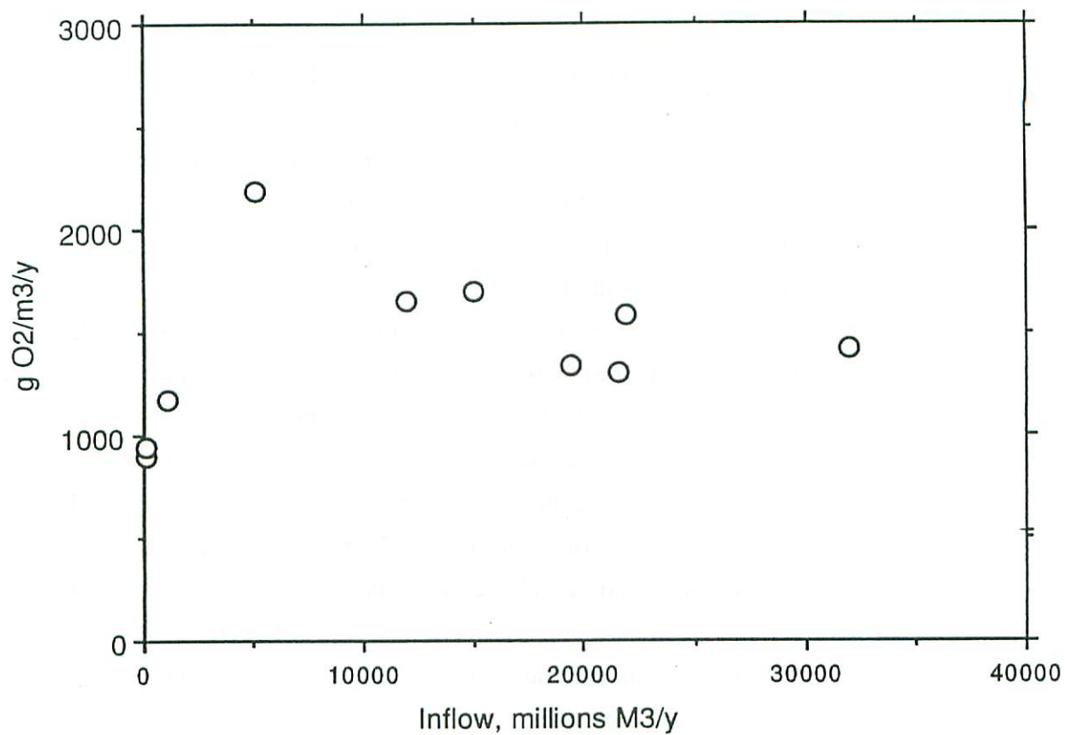
Figure 21. Annual community production, g O 2 /M 3 /y, in Nueces and Trinity bays, vs estuary inflow. Three Nueces Bay points are at lower left.
