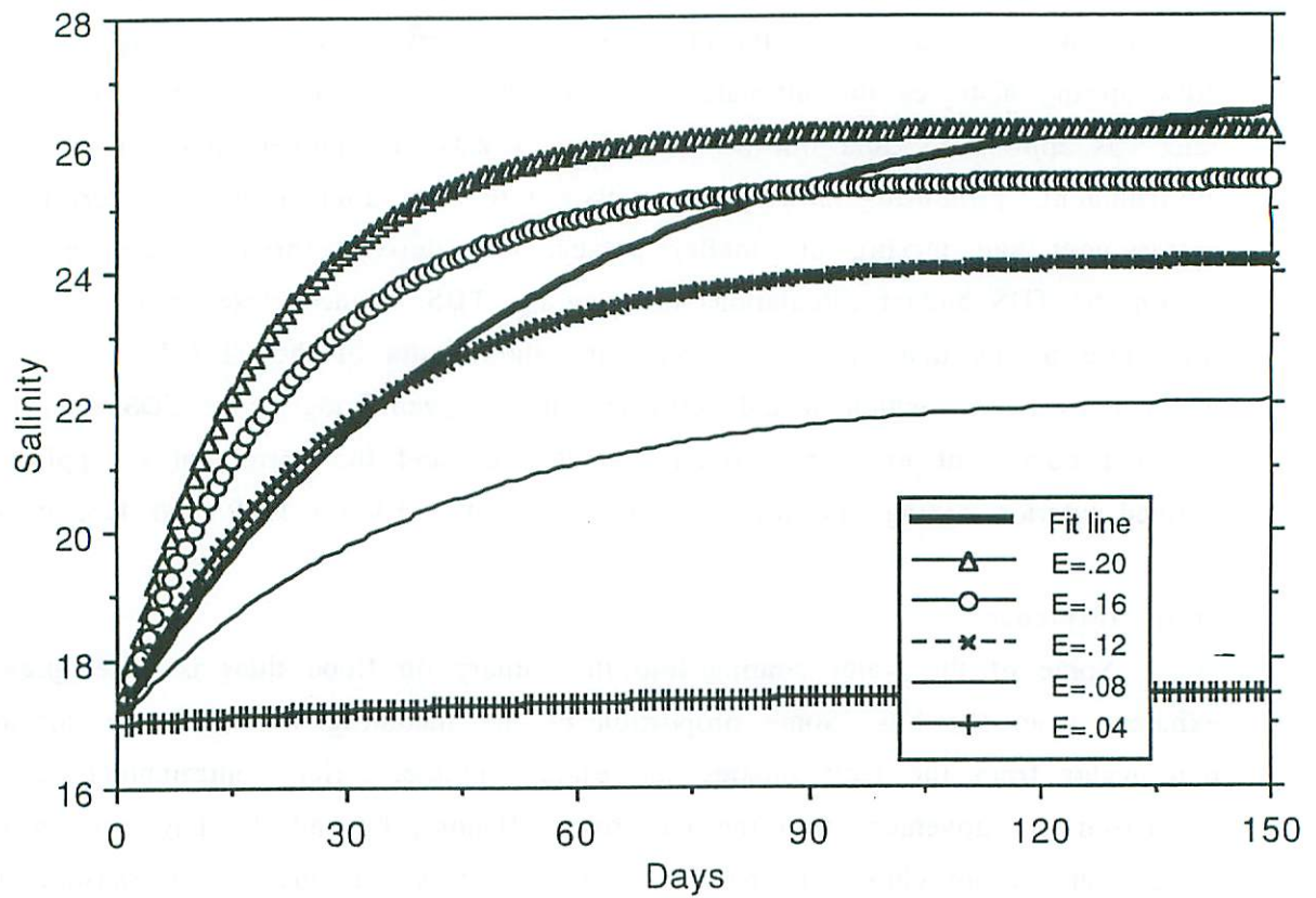
Figure. 3 Salinity recovery, fit line vs recovery calculated using trial entrainment rates, Dollar Point.
