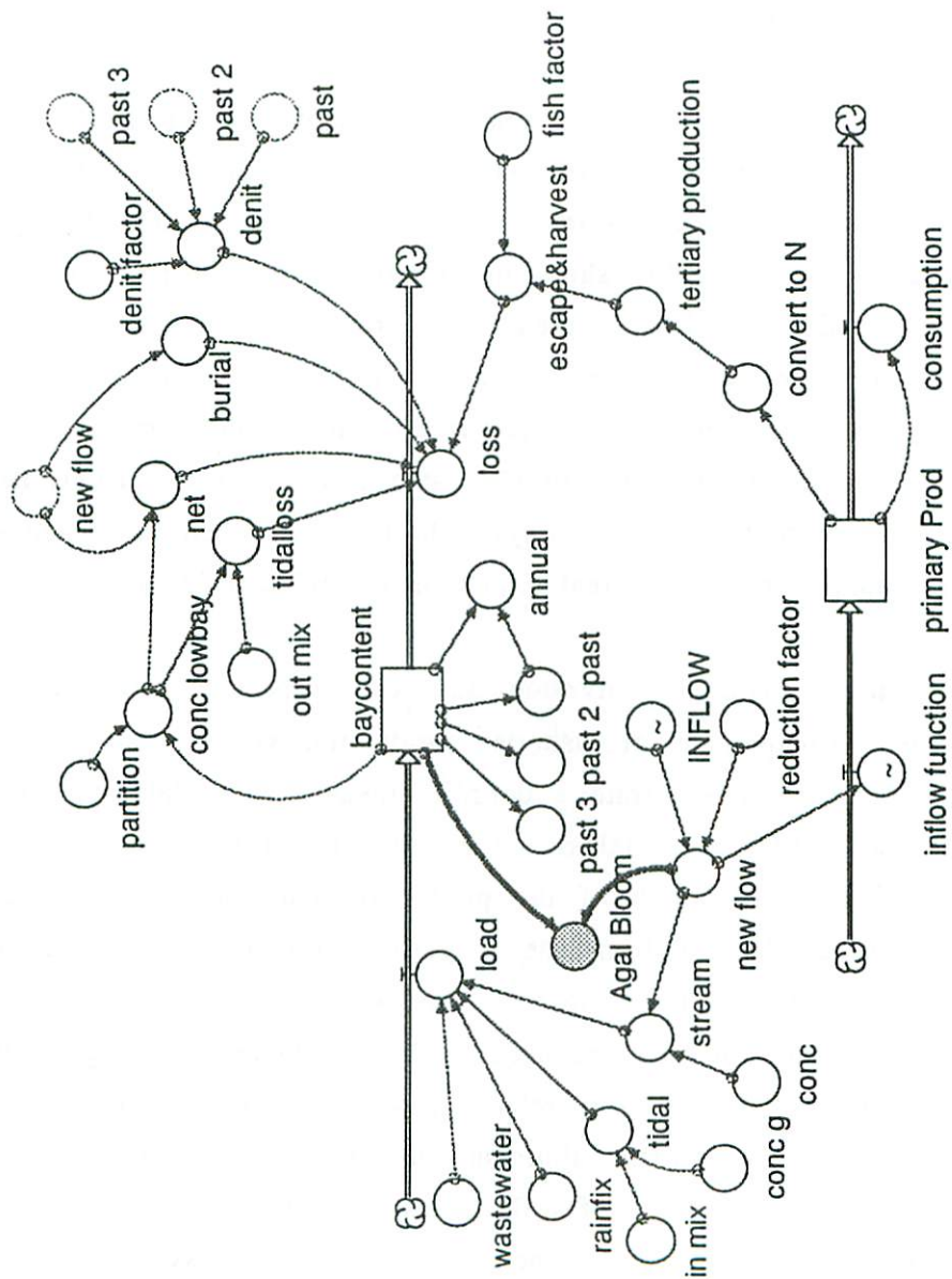
Figure 32. Model diagram showing module for indication of conditions promoting algal bloom formation.
