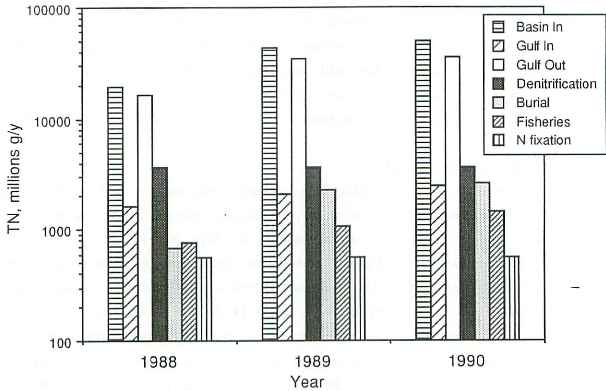
Figure 7. Comparison of TN inputs and losses, Galveston Bay. Note log scale.
