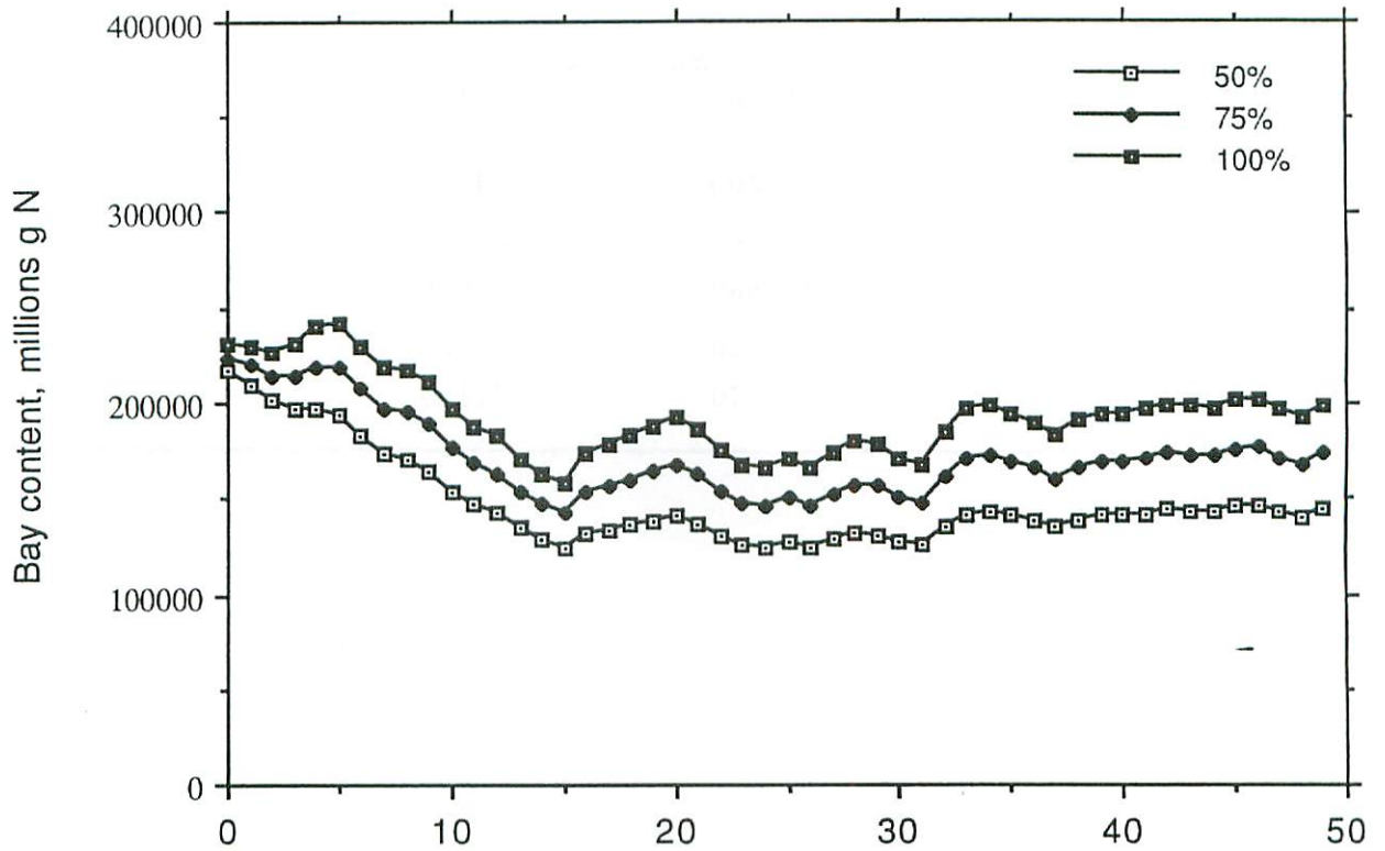
Figure 30. Bay content sensitivity to reduction in freshwater inflows. Inflows as percentage of normal.
