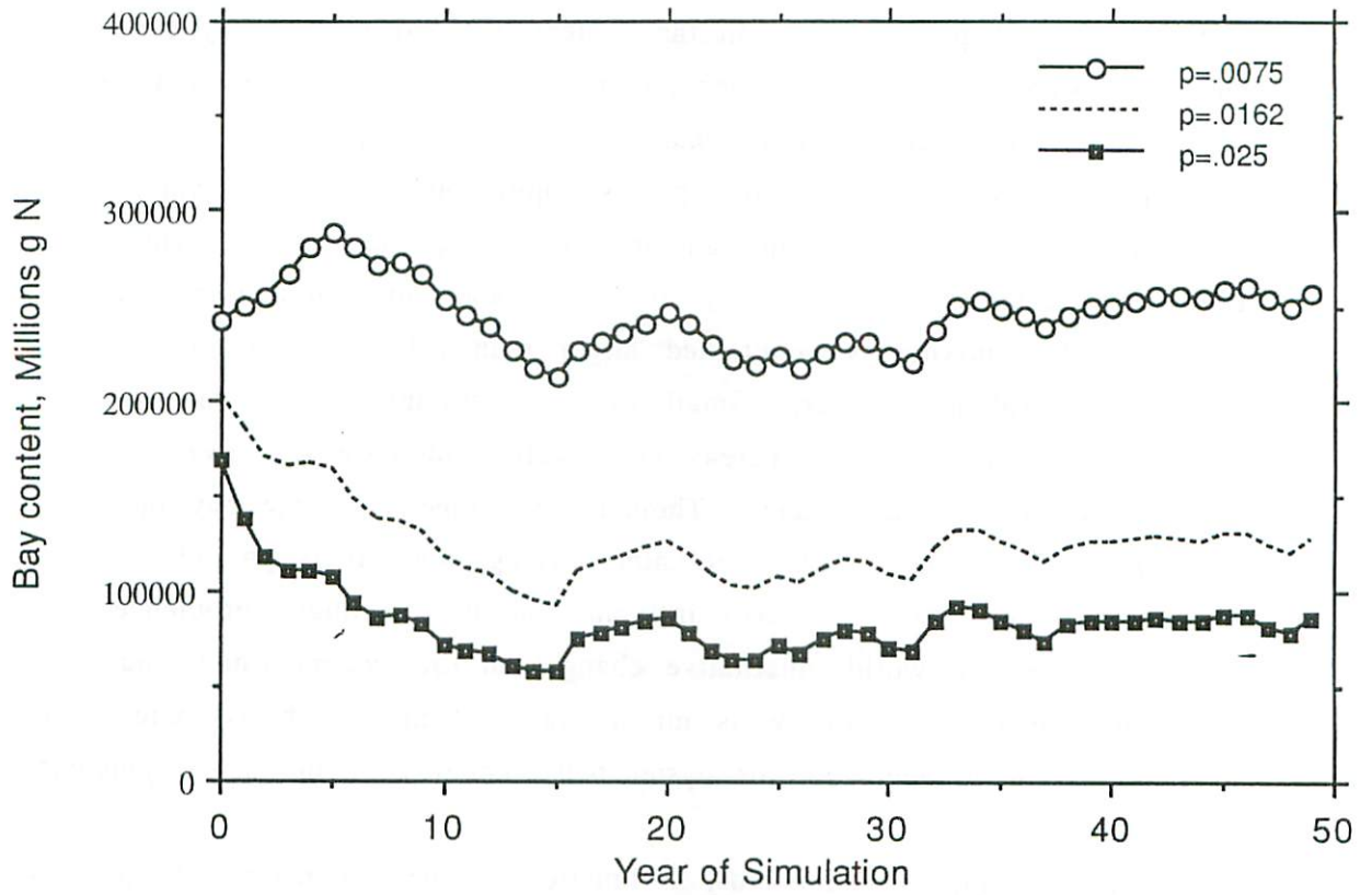
Figure 29. Sensitivity of bay content to the partition coefficient.
