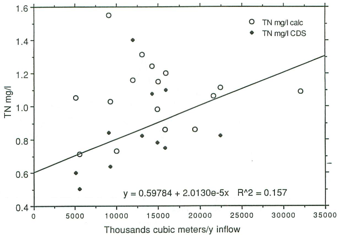
Figure 5. Variation of lower Galveston Bay TN with inflow. CDS points are TN = TKN + NO_3 + NO_2 , others from regression on NO_3 + NO_2 + NH_3 . Line is fit through CDS points.
