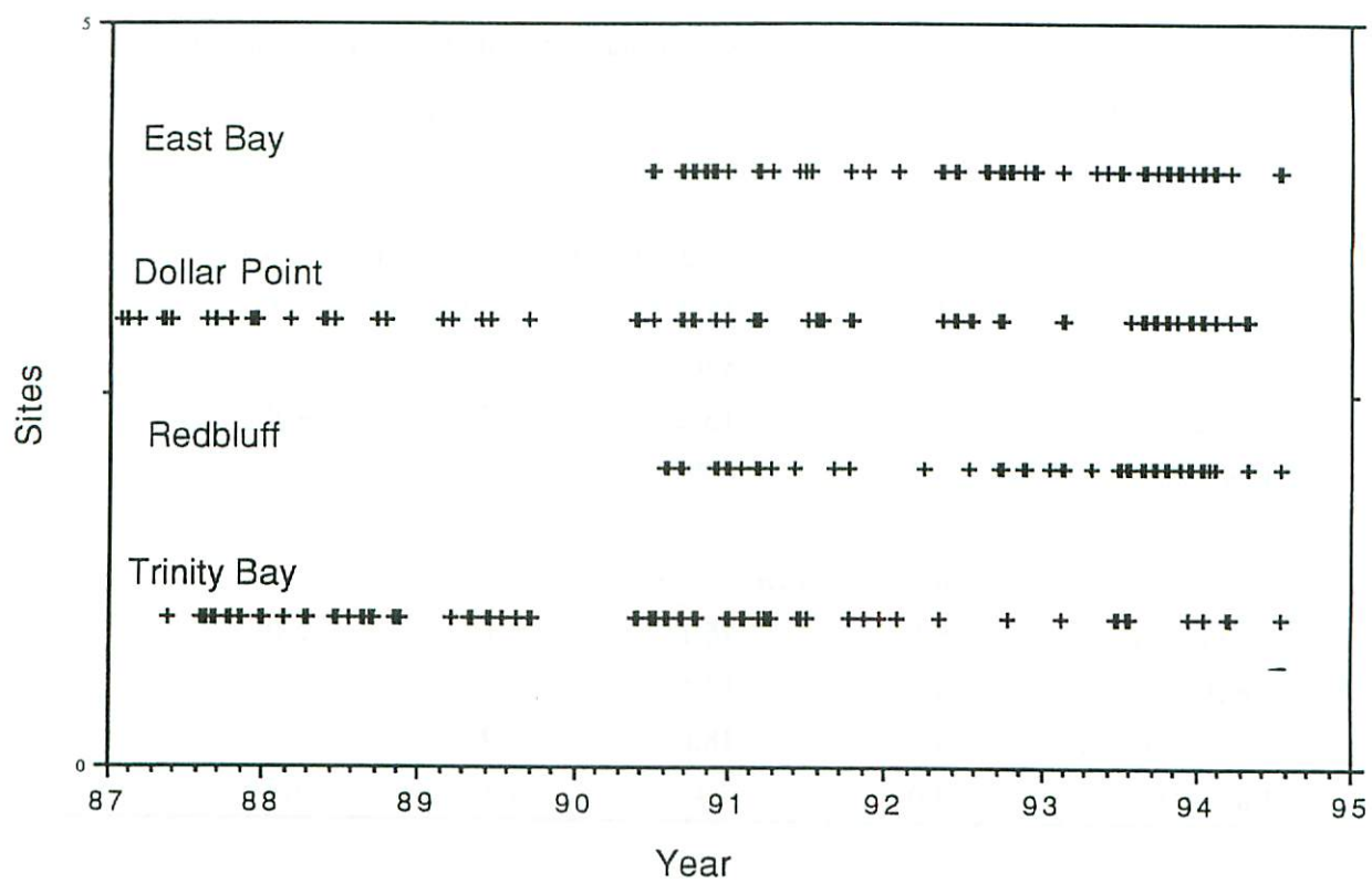
Figure 16. Dates with measurements of diurnal metabolism for each Galveston Bay site
