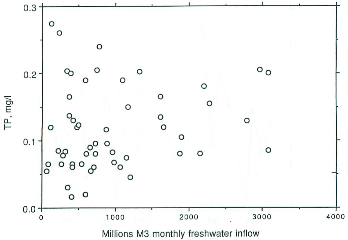
Figure 10. Total Phosphorus concentrations in lower Galveston Bay vs inflows.
