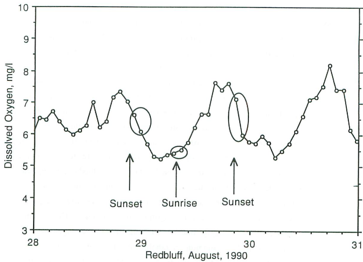
Figure 14. Adjacent measurements averaged in calculations of diffusion and respiration rates.
