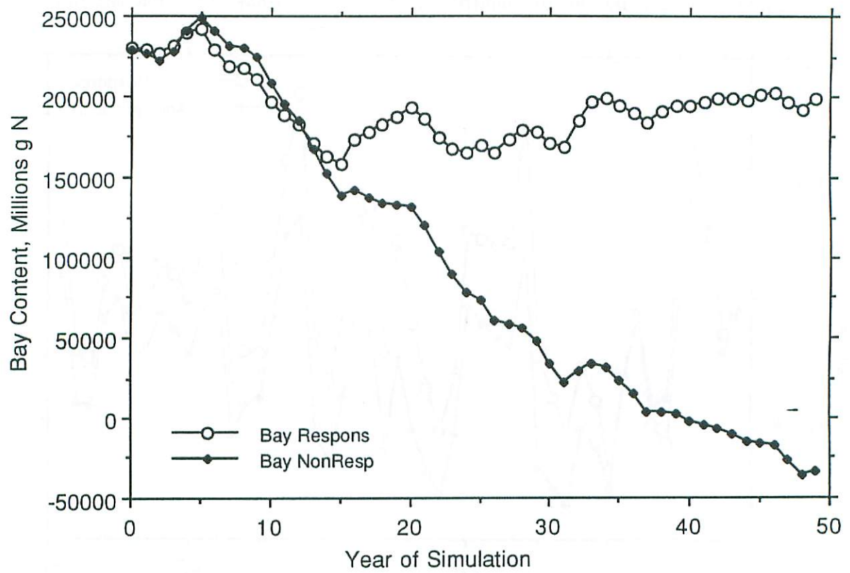
Figure 27. Sensitivity of bay content to incorporating feedback from bay content in calculation of denitrification and lower-bay TN concentration.
