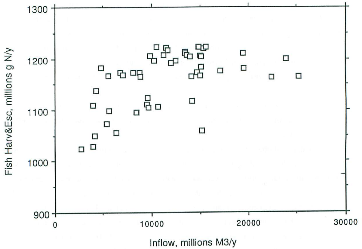
Figure 23 Relationship of nitrogen loss via fisheries to freshwater inflow volume in simulation results.
