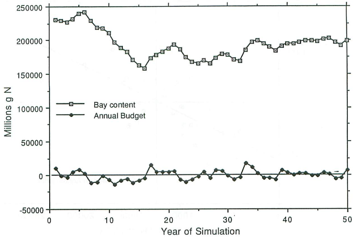
Figure 24. Annual nitrogen balance and bay nitrogen content simulated over 50 years, using 1941-1990 inflows.
