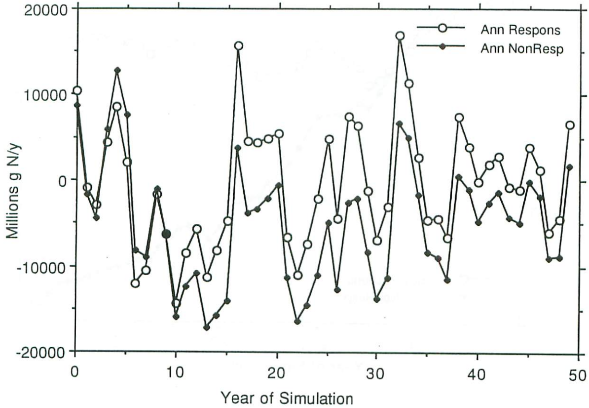
Figure 26. Sensitivity of annual balance to incorporating feedback from bay content in calculation of denitrification and lower-bay TN concentration.
