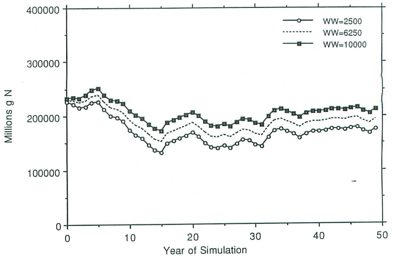
Figure 28. Baycontent sensitivity to wastewater input variation.
