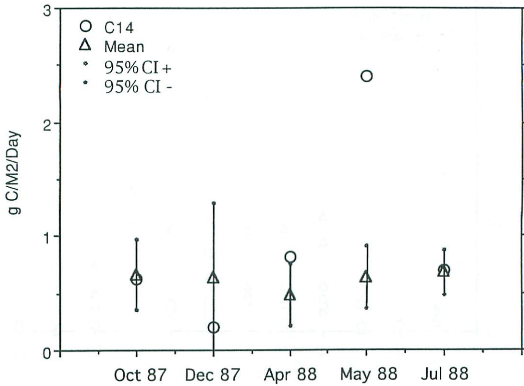
Figure 18. Comparison between production measurements in Nueces Bay by ^{14}\text{C} and diurnal oxygen curve techniques.
